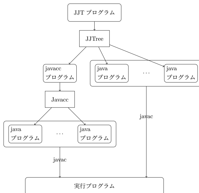
図 4.3: jjtree-config
