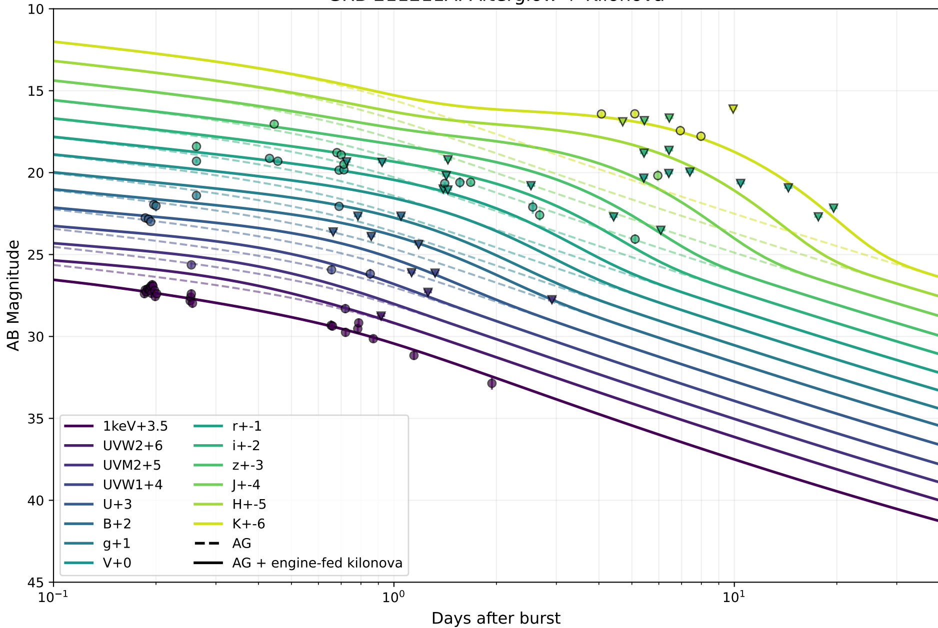
GRB 211211A: Afterglow + Kilonova
