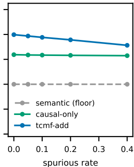
spurious edges (realistic pool, 5-seed 95% CI)
