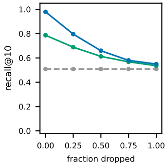
edge dropout (small pool, single run)
