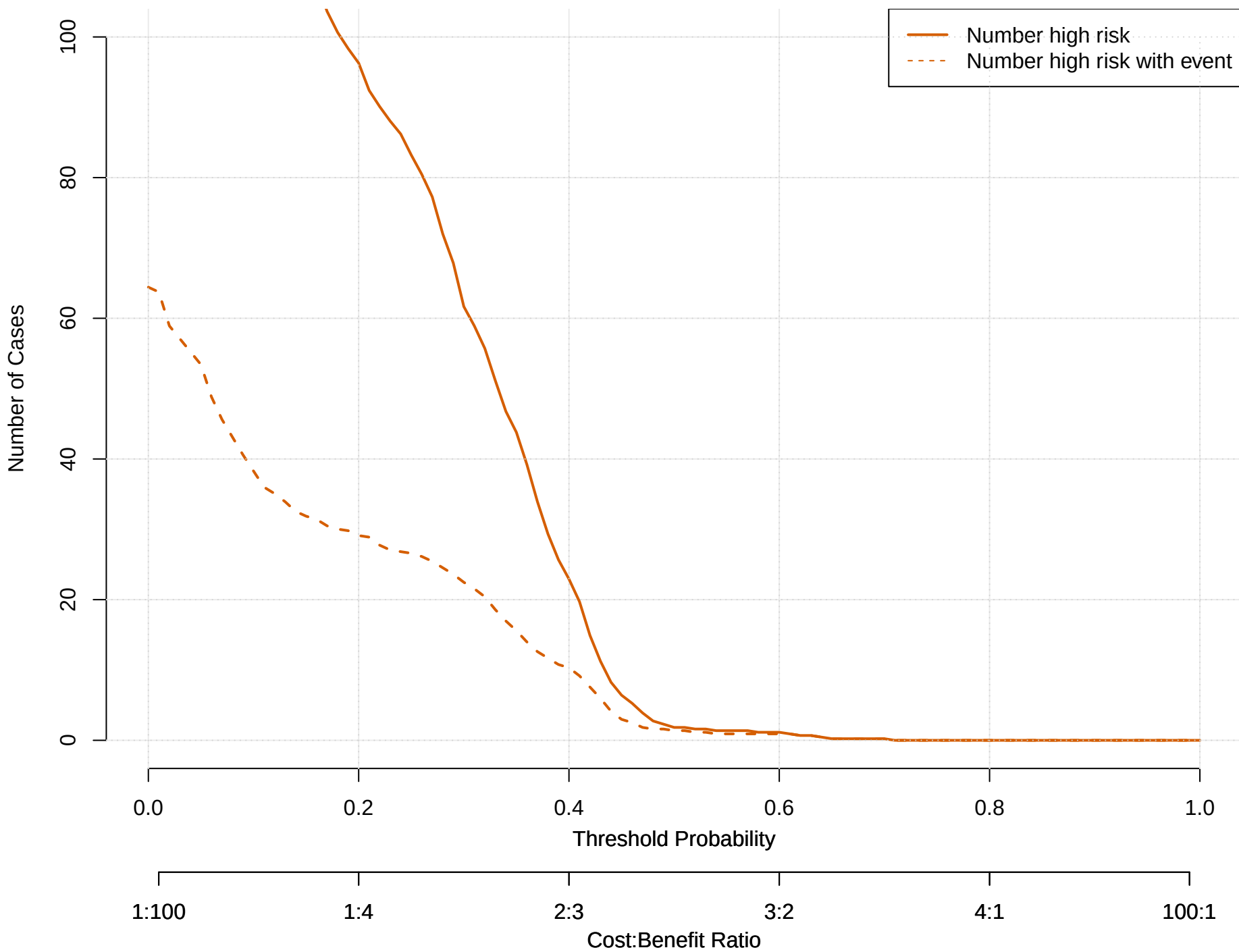
Clinical Impact Curve – MLP
