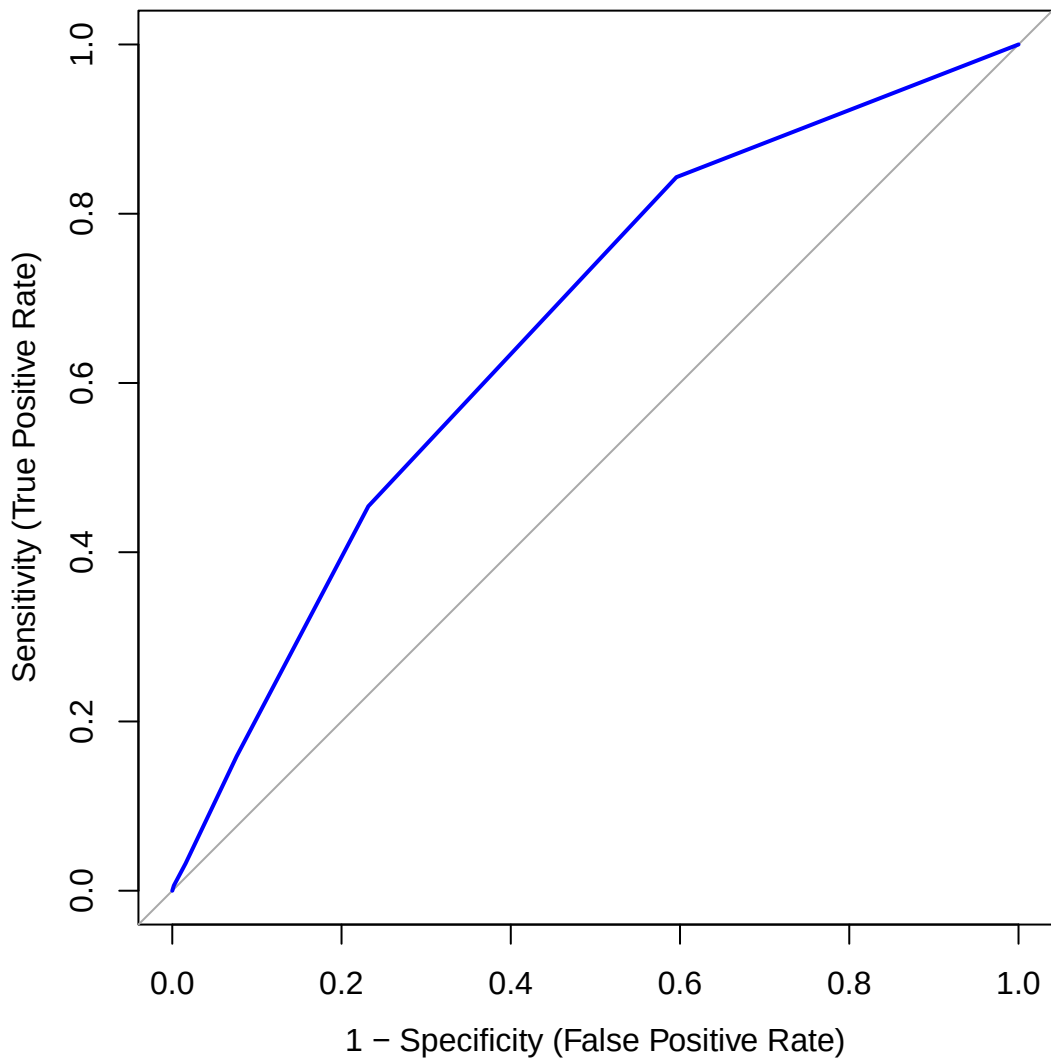
ROC Curve – MDS1 (AUC = 0.662 )
