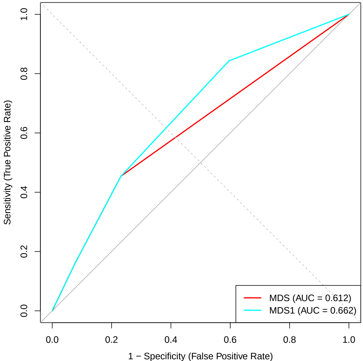
ROC Curves for Different Exposures
