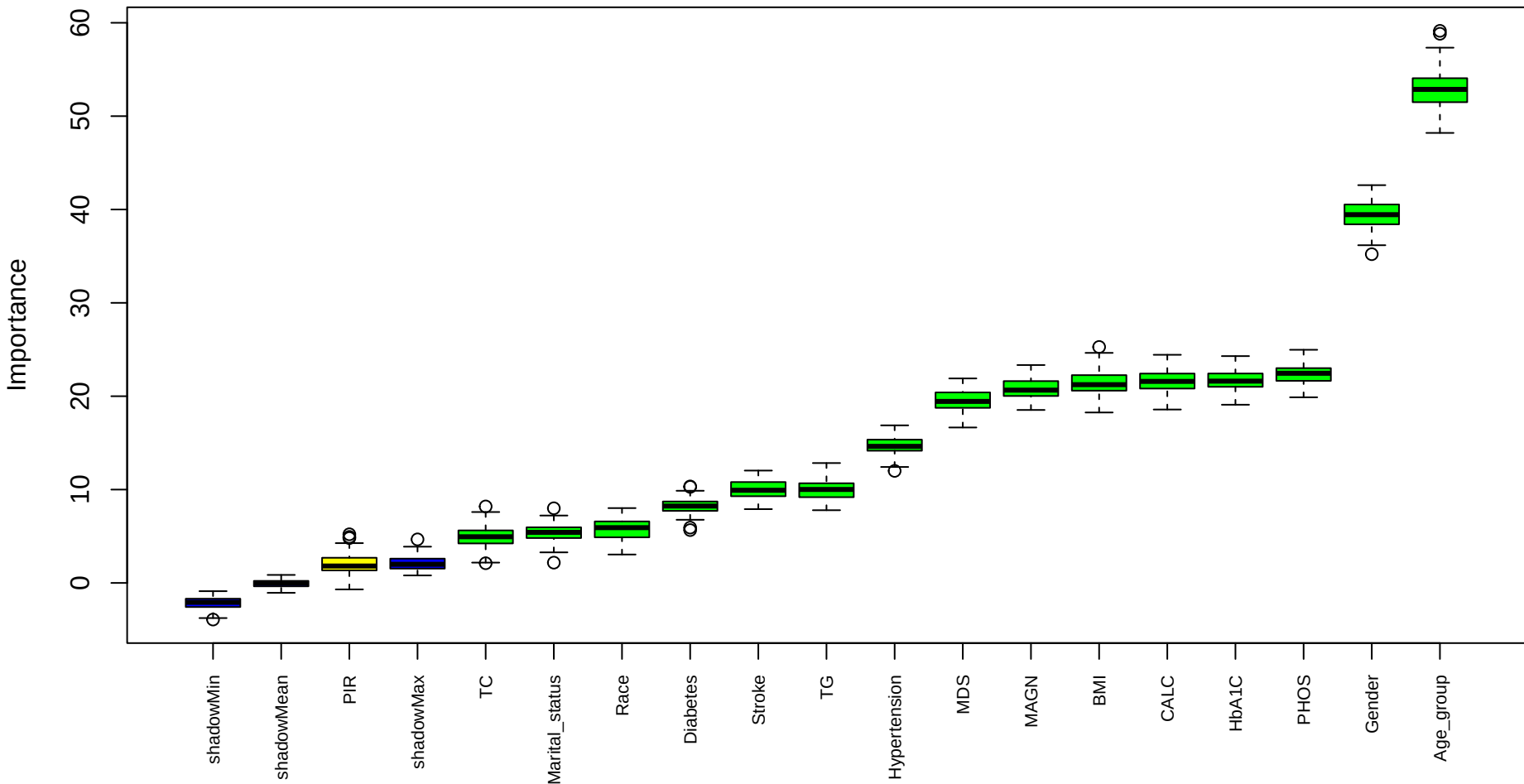
Boruta Feature Importance
