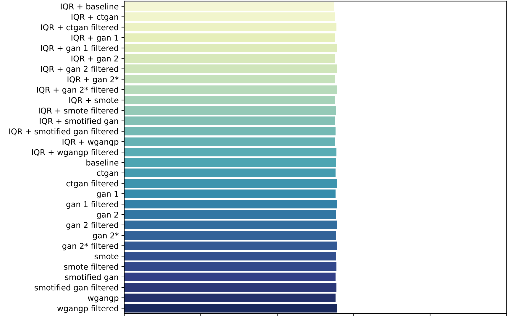
WeatherAUS
