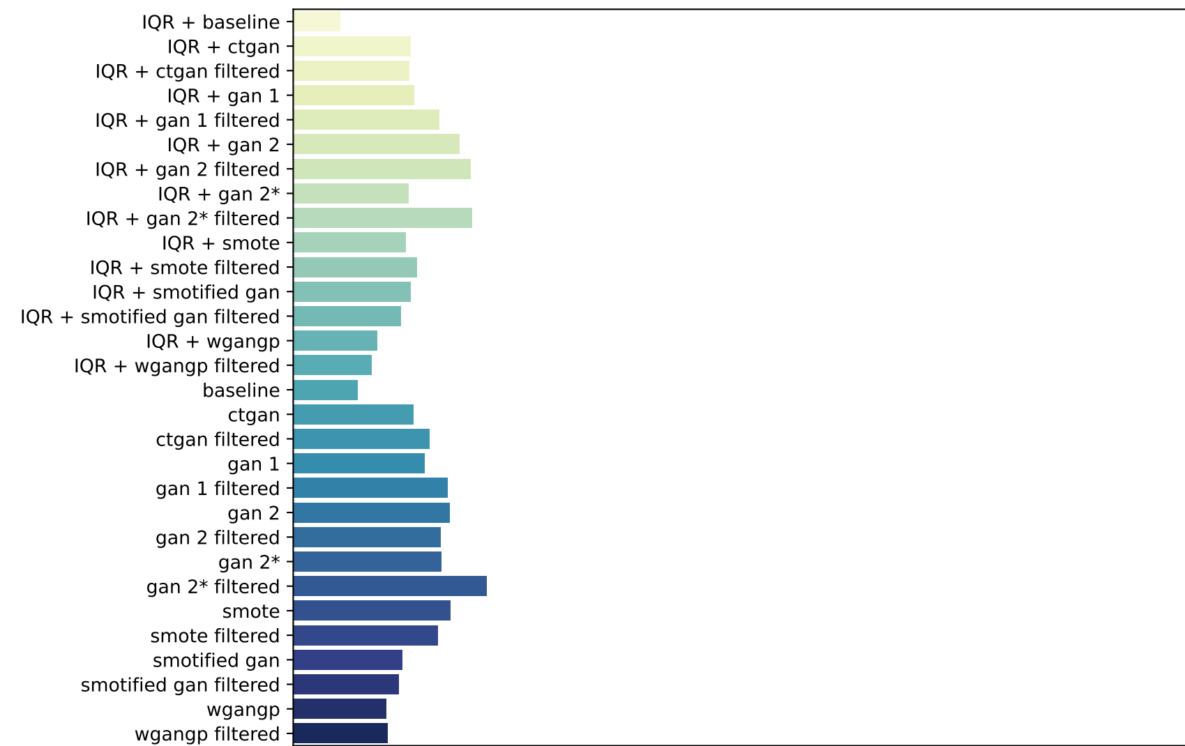
Ionosphere
