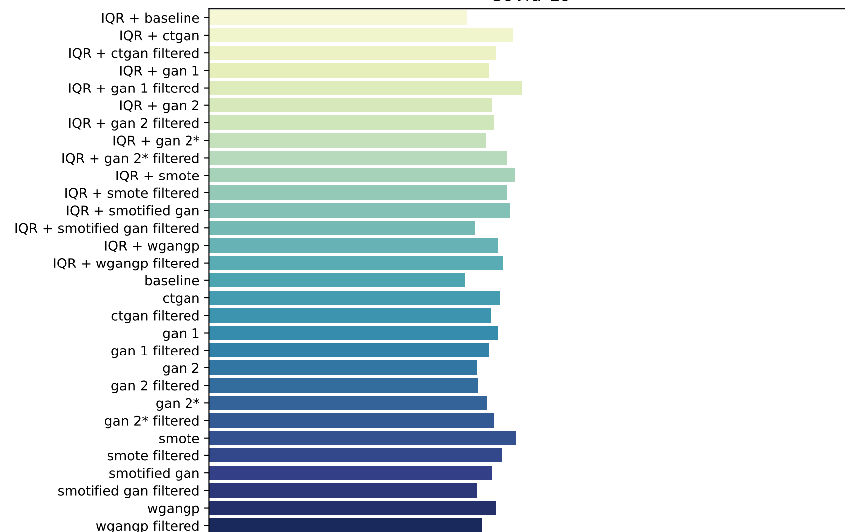
Haberman's Survival
