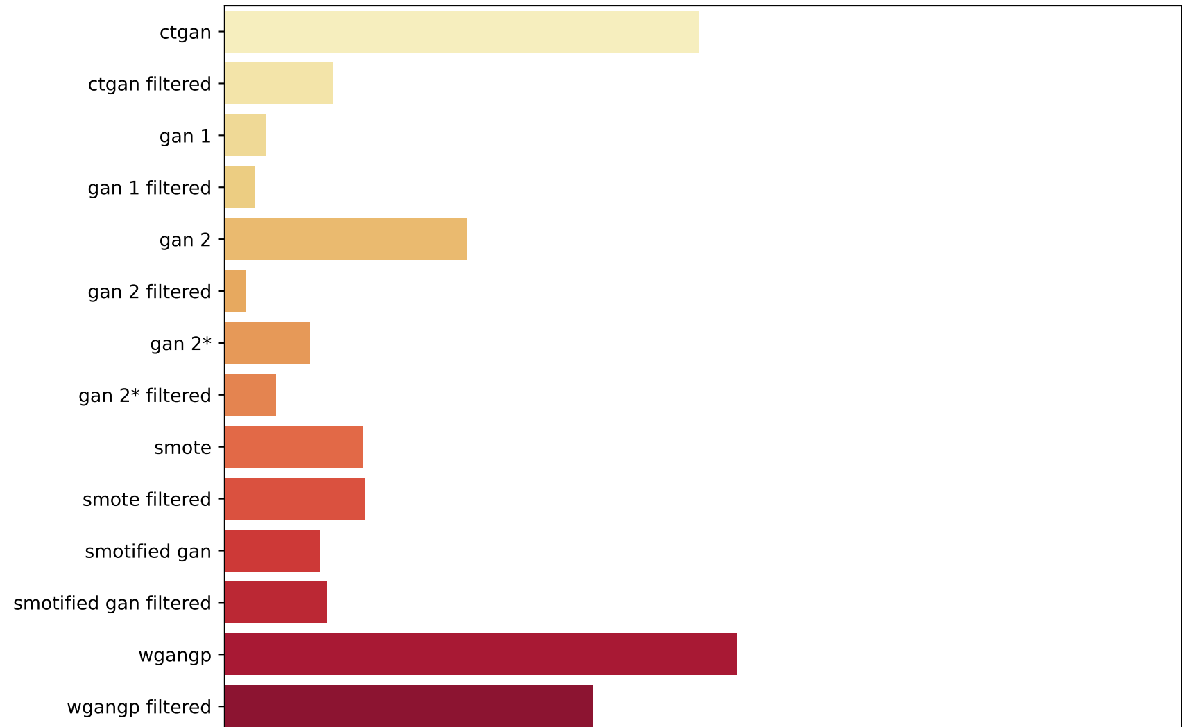
IQR Banknote
