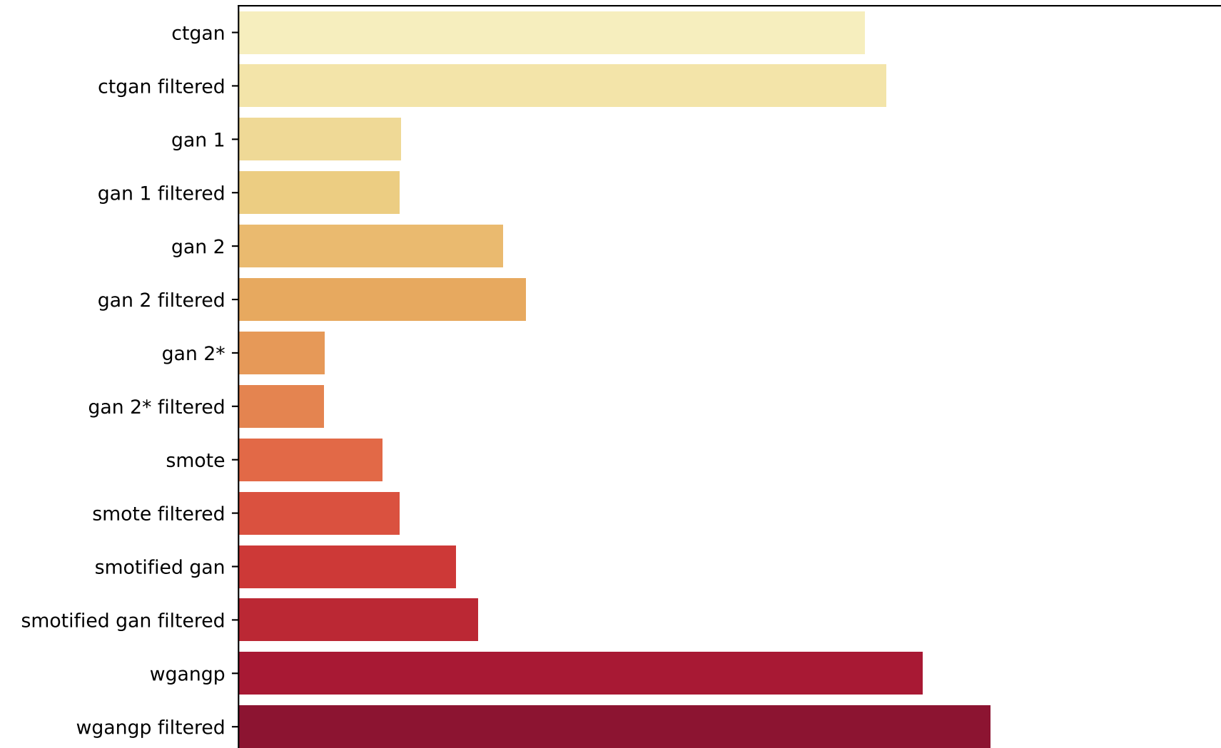
Sonar
