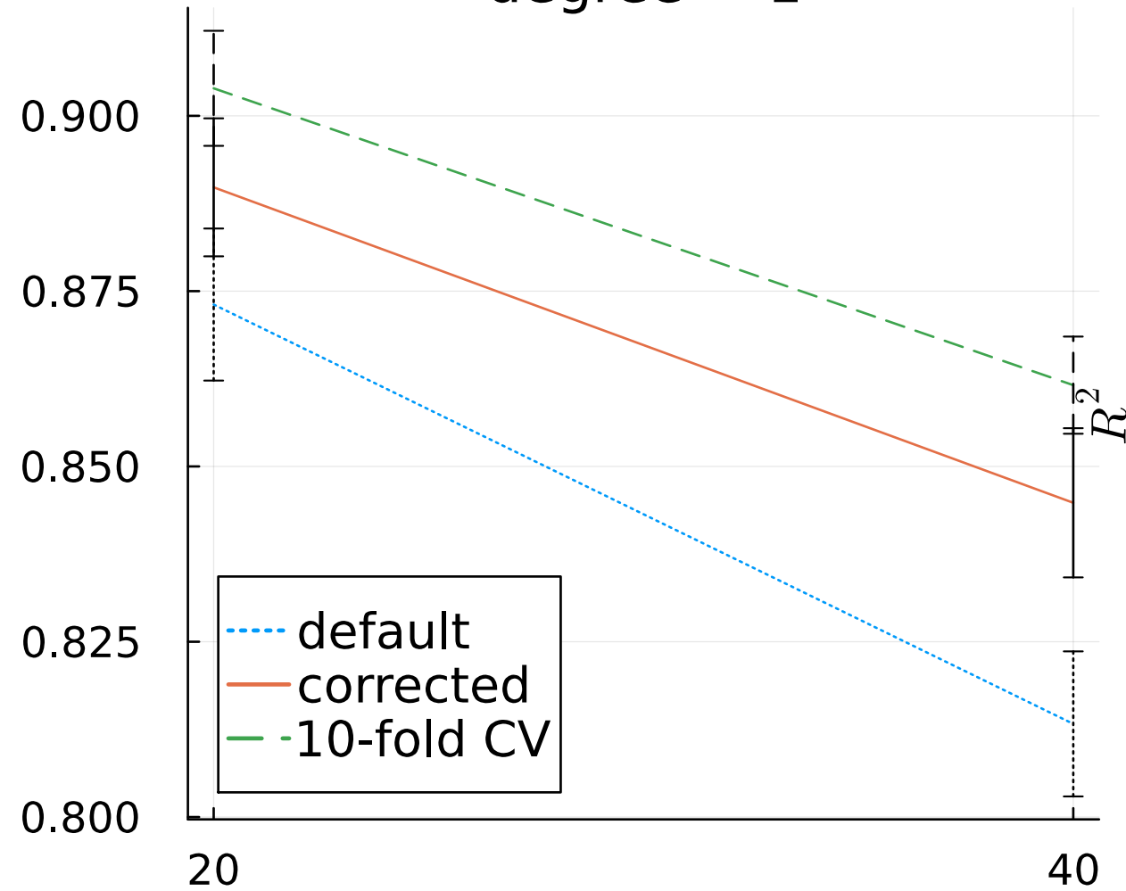
degree = 1
