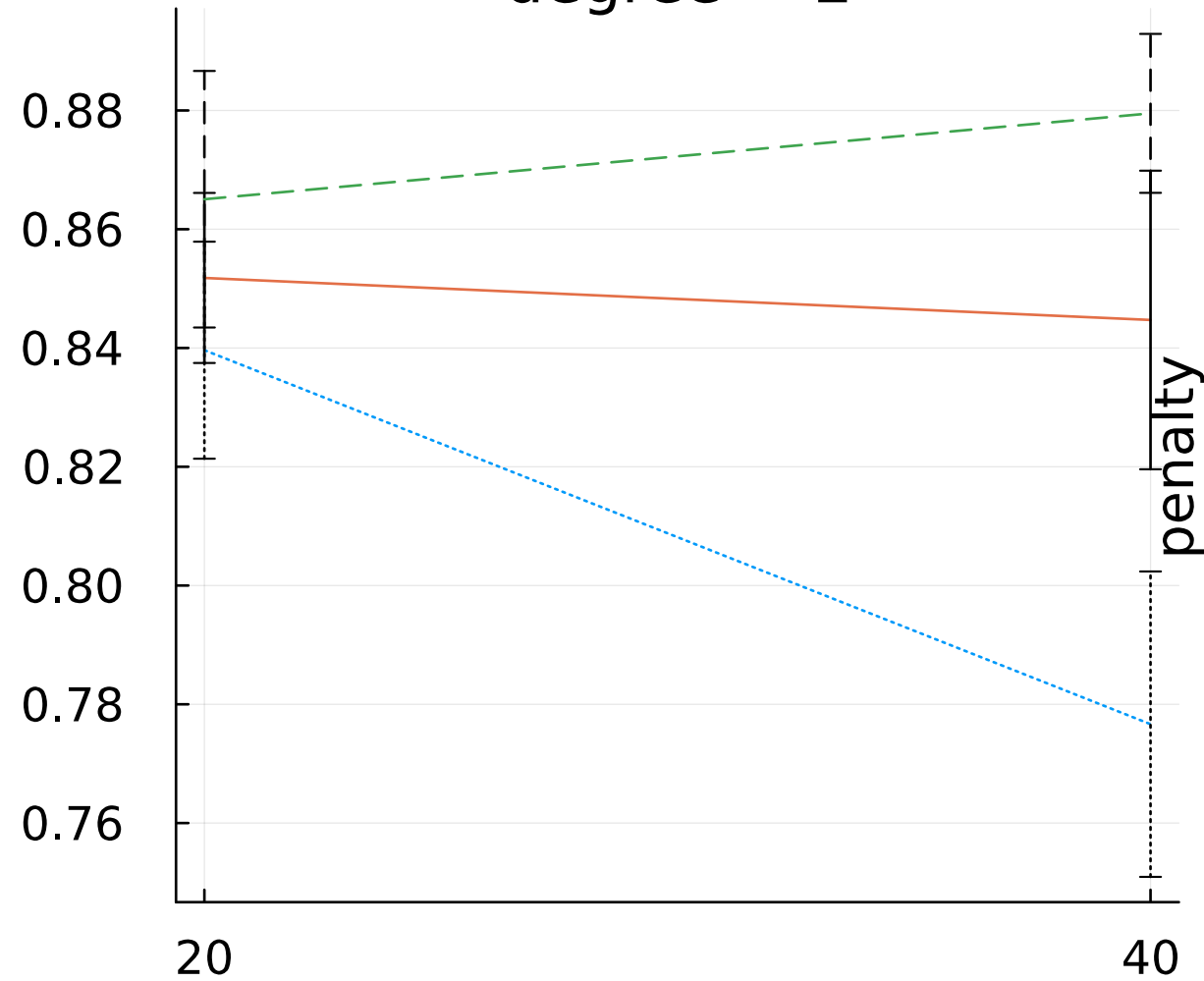
degree = 2
