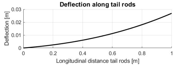
Figure 13: Deflection tail rods.
