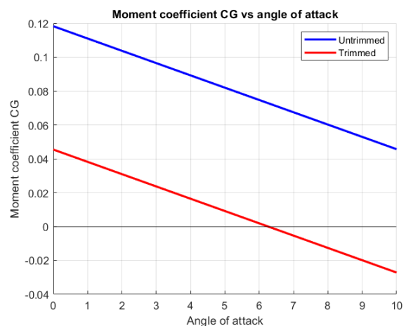
Figure 10: Moment coefficient about CG vs angle of attack
