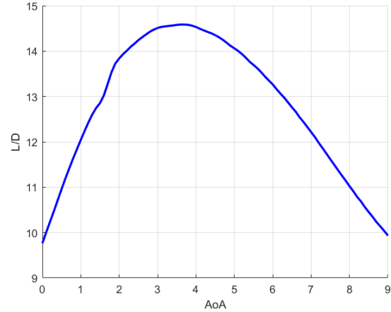
Figure 4: Lift over drag ratio for geometric angles of attack.
