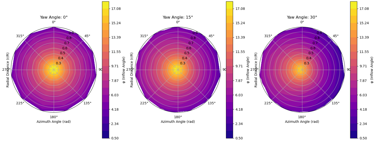
Figure 18: Contour plot showing variation of flow angle \phi along the spanwise distribution for the three yaw angles \theta_{yaw} = 0^\circ, 15^\circ, 30^\circ .
