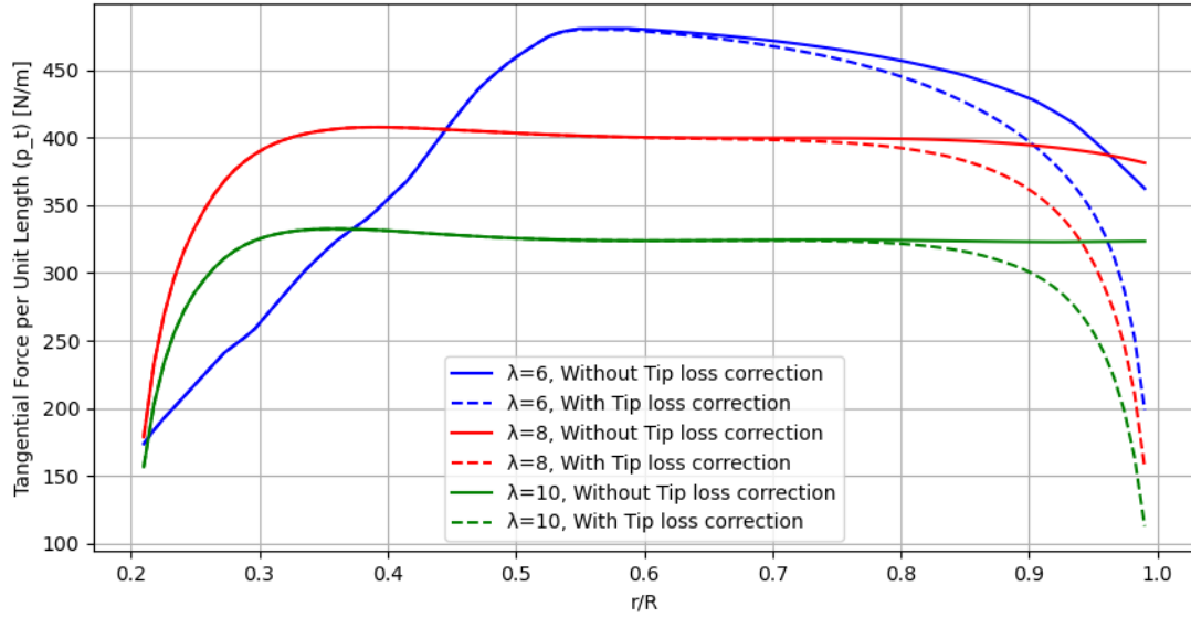
Figure 10: Spanwise distribution of azimuthal load p_t with and without Prandtl's tip correction for \lambda = 6, 8, 10 .
