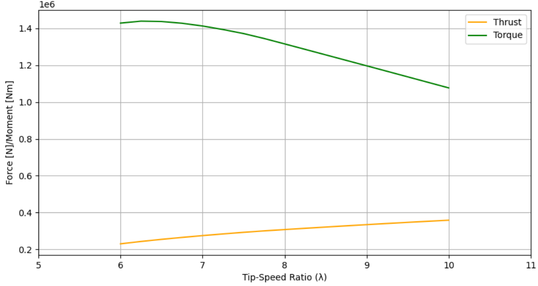
Figure 8: Total thrust and torque for tip speed ratio range \lambda = 6 - 10 .
