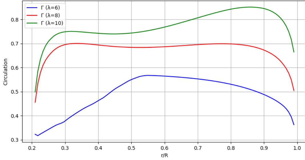
Figure 13: Spanwise distribution of circulation \Gamma for tip speed ratio \lambda = 6, 8, 10 .
