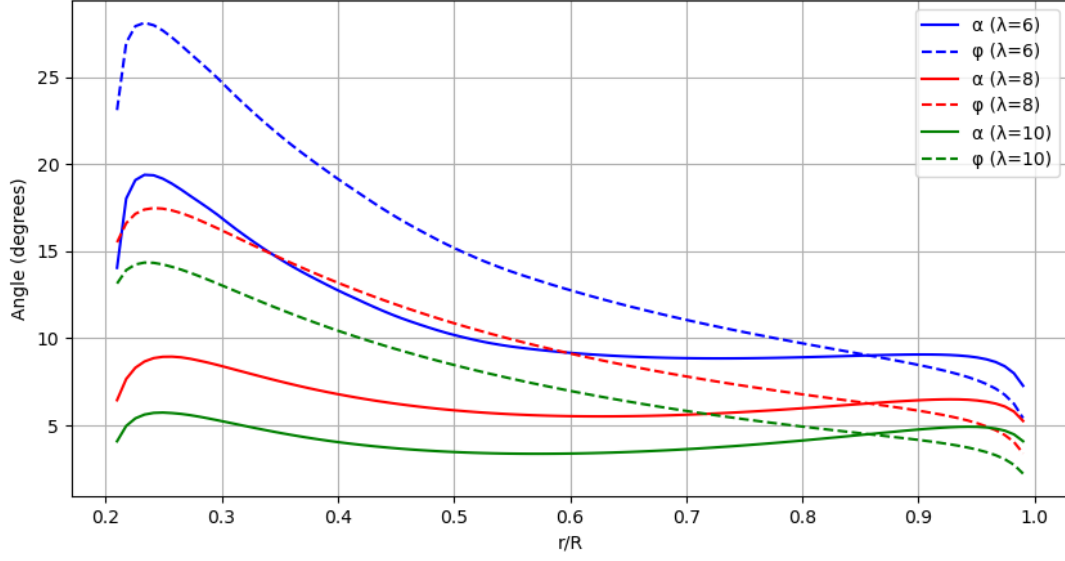
Figure 5: Spanwise distribution of angle of attack \alpha and inflow angle \phi for tip speed ratio \lambda = 6, 8, 10
