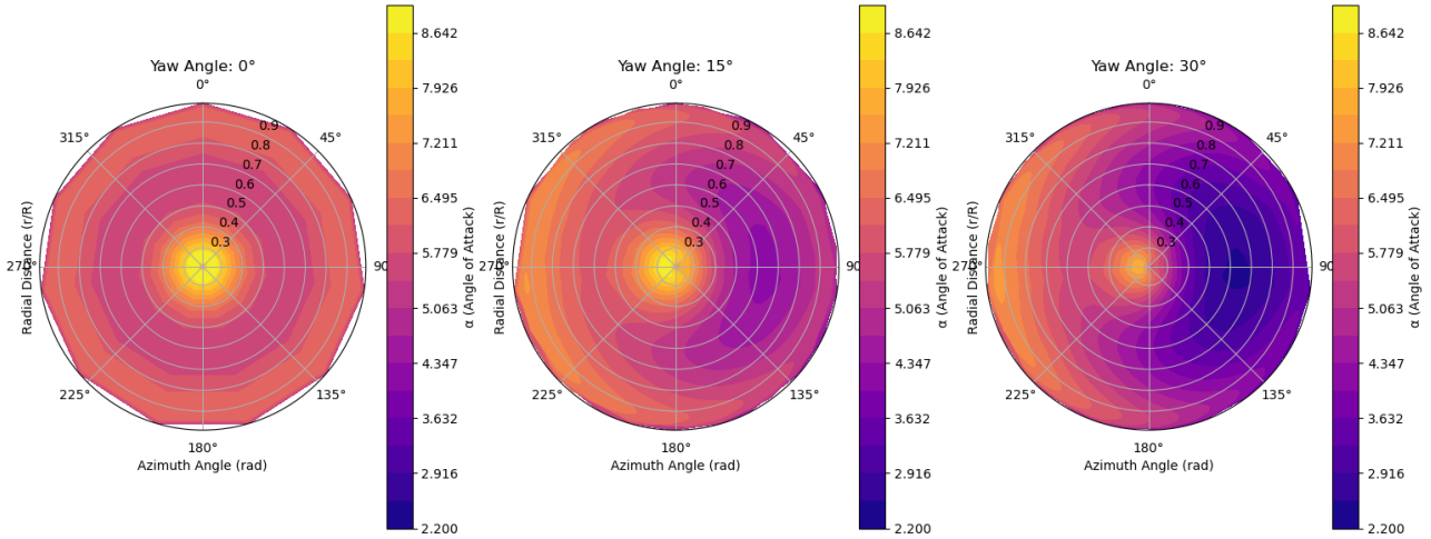
Figure 17: Contour plot showing variation of angle of attack \alpha along the spanwise distribution for the three yaw angles \theta_{yaw} = 0^\circ, 15^\circ, 30^\circ .
