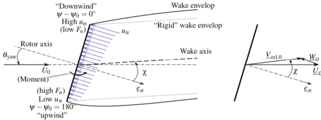
Figure 14: Yawed configuration and resulting velocity triangle. Adapted from [1]
