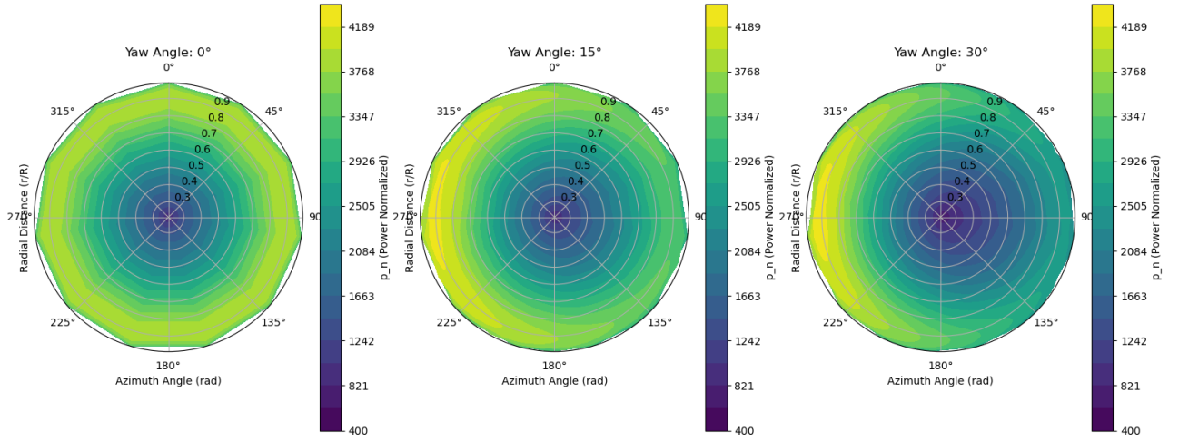
Figure 19: Contour plot showing variation of normal load p_n along the spanwise distribution for the three yaw angles \theta_{yaw} = 0^\circ, 15^\circ, 30^\circ .
