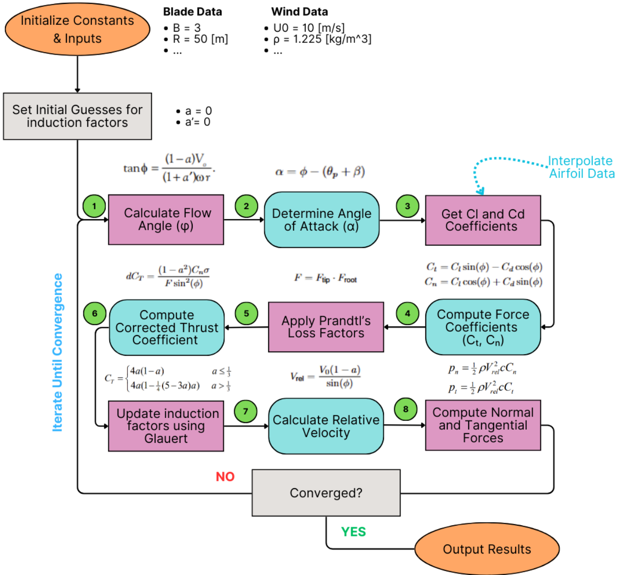
Figure 2: Blade Element Method Algorithm represented in a Flowchart.
