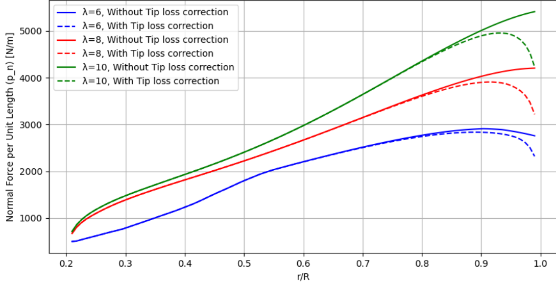
Figure 9: Spanwise distribution of axial load p_n with and without Prandtl's tip correction for \lambda = 6, 8, 10 .
