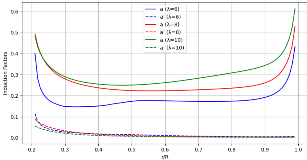
Figure 6: Spanwise distribution of axial and azimuthal induction factors a, a' for tip speed ratio \lambda = 6, 8, 10
