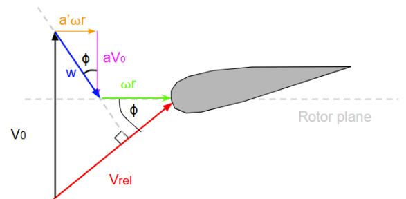
Figure 1: Velocity triangle at a blade element, showing the effect of induced velocities ( a , a' ) on the relative wind speed and inflow angle.
