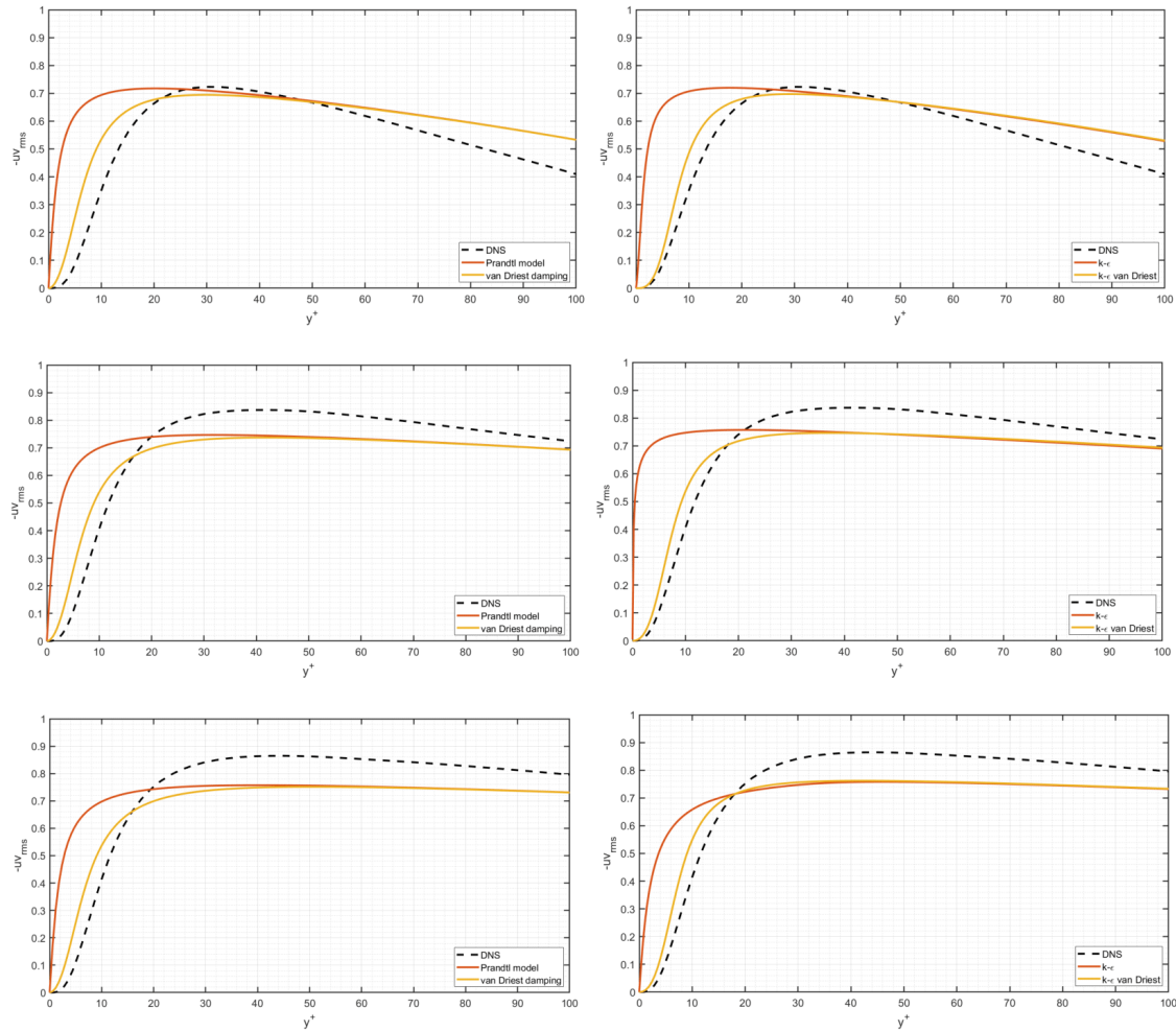
Figure 2: Reynolds shear stress -\overline{u'v'} normalized by the wall shear velocity in wall coordinates — Damped Prandtl/ k - \epsilon , — Undamped Prandtl/ k - \epsilon , — DNS; for Re_\tau = 180 (Row 1), Re_\tau = 395 (Row 2), Re_\tau = 590 (Row 3).
