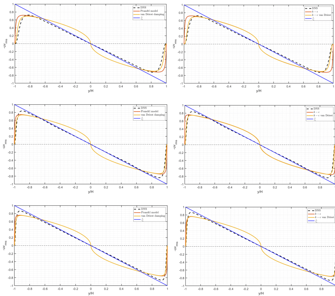
Figure 3: Reynolds shear stress -\overline{u'v'} normalized by the wall shear velocity in global coordinates — Damped Prandtl/ k - \epsilon , — Undamped Prandtl/ k - \epsilon , — DNS; for Re_\tau = 180 (Row 1), Re_\tau = 395 (Row 2), Re_\tau = 590 (Row 3).
