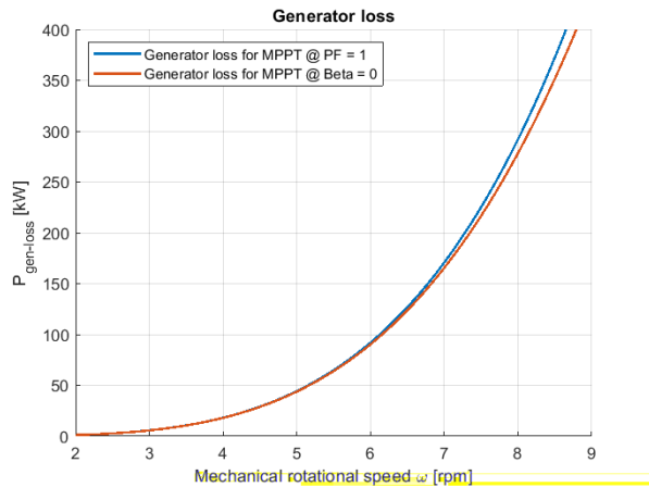
Figure 5: Generator loss as a function of Mechanical rotational speed \omega
