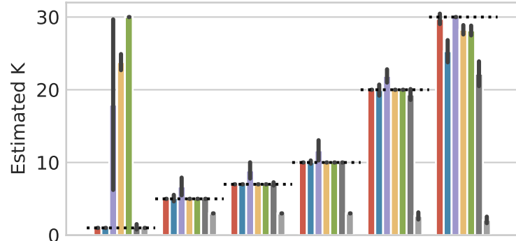
Varying number of factors
