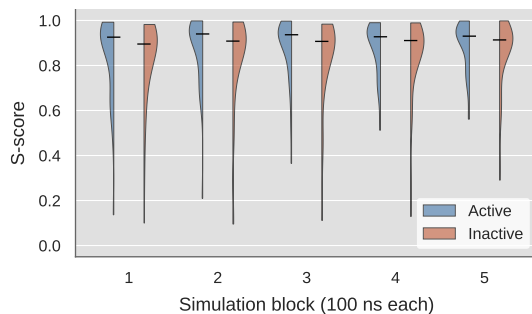
(b) S-score: activity cliffs
