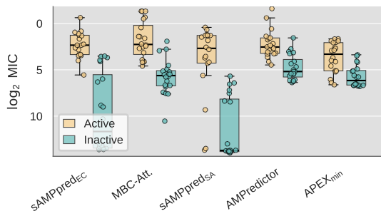
(g) ML regressors: control dataset
