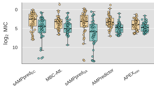
(h) ML regressors: activity cliffs
