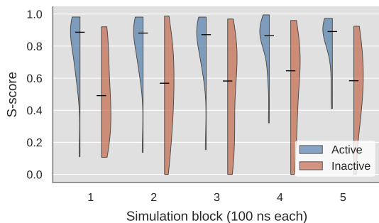
(a) S-score: control dataset
