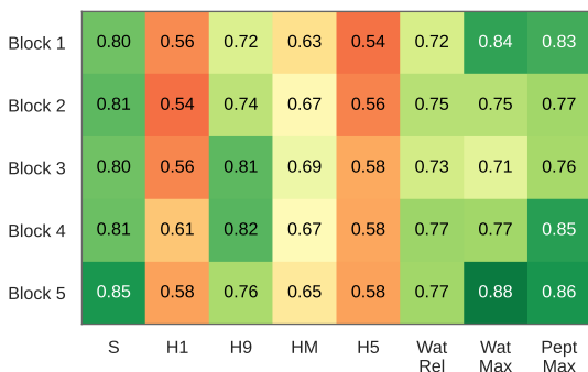
(c) AUC by descriptor: control dataset
