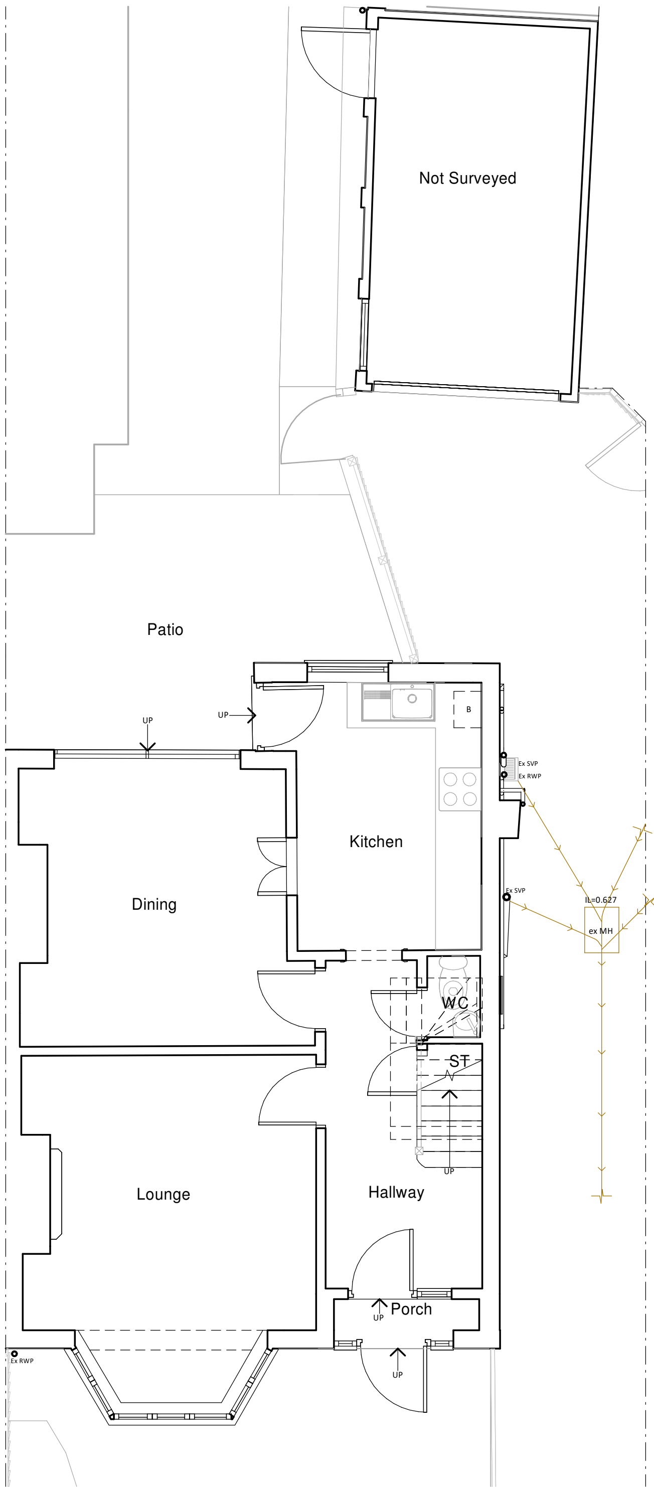
Ground Floor Plan Area ca. 43.20 m²
