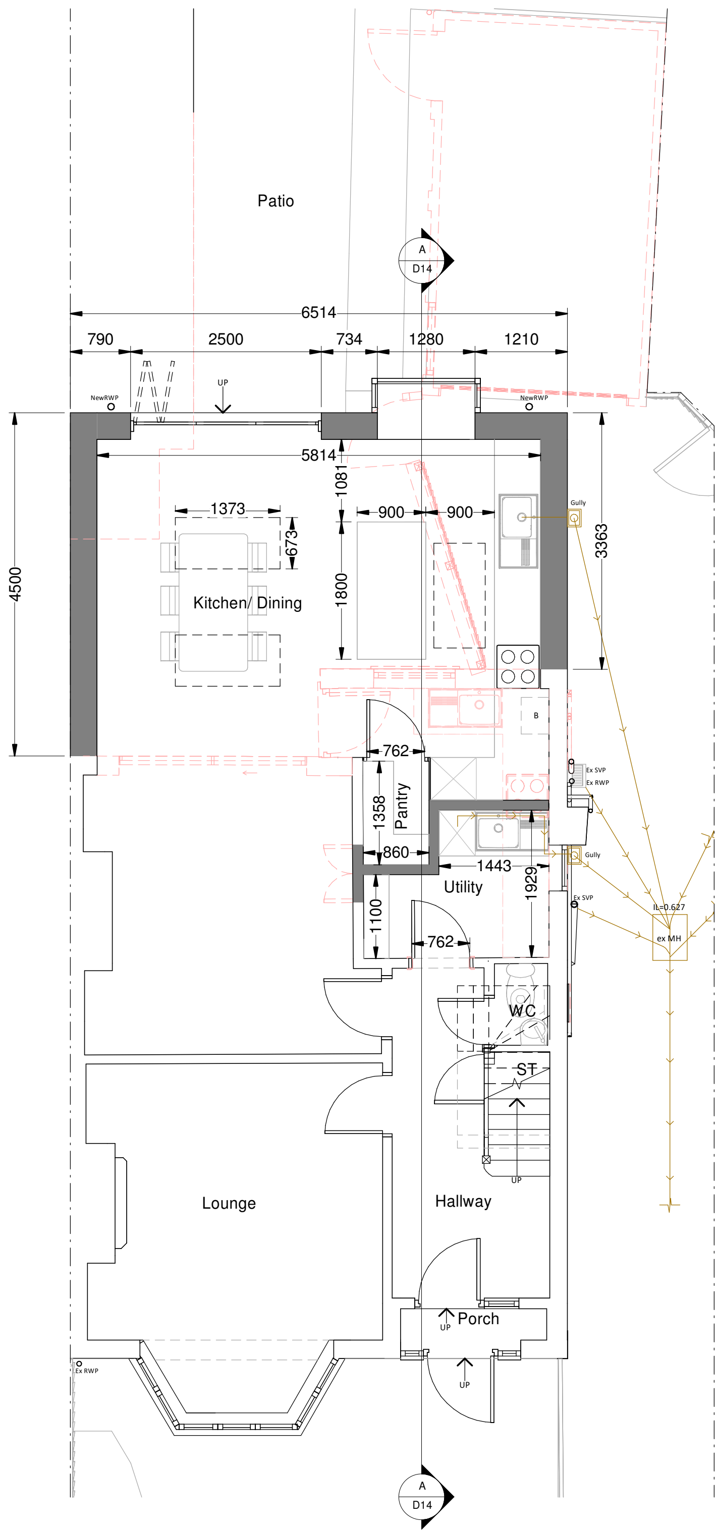
Ground Floor Plan Area ca. 43.20 m 2 Additional Area: 22.40 m 2
