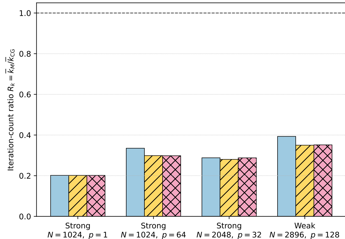
(a) Iteration-count ratio
