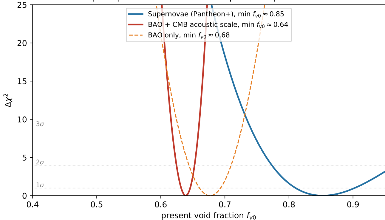
Timescape: supernovae and BAO+CMB require incompatible void fractions
