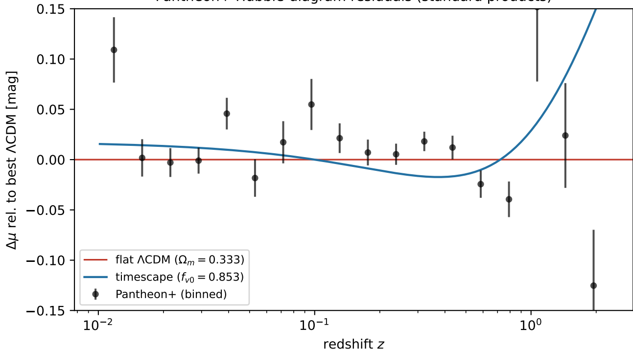
Pantheon+ Hubble-diagram residuals (standard products)
