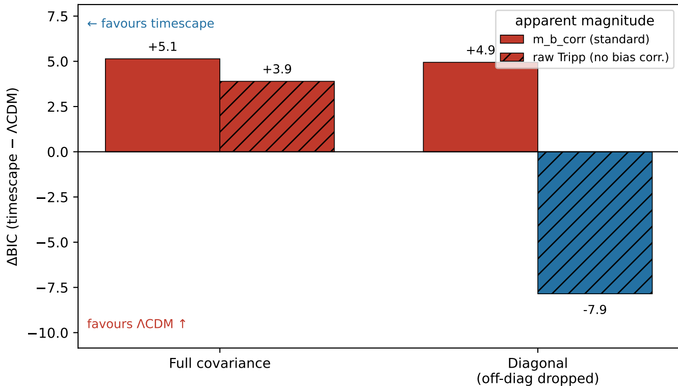
Timescape is preferred only when the off-diagonal covariance is dropped
