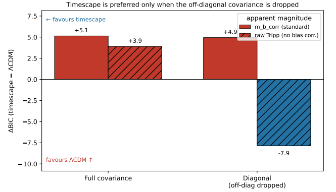
FIG. 1. Model-comparison verdict on Pantheon+ across magnitude (solid = m_{B,\text{corr}} , hatched = raw Tripp) and covariance (full vs diagonal). Red favours \Lambda CDM, blue favours timescape. Only the raw-Tripp+diagonal case favours timescape; the full covariance favours \Lambda CDM for every magnitude definition.
