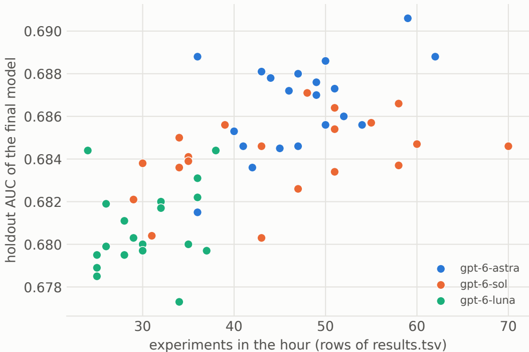
Experiments per run against holdout AUC
