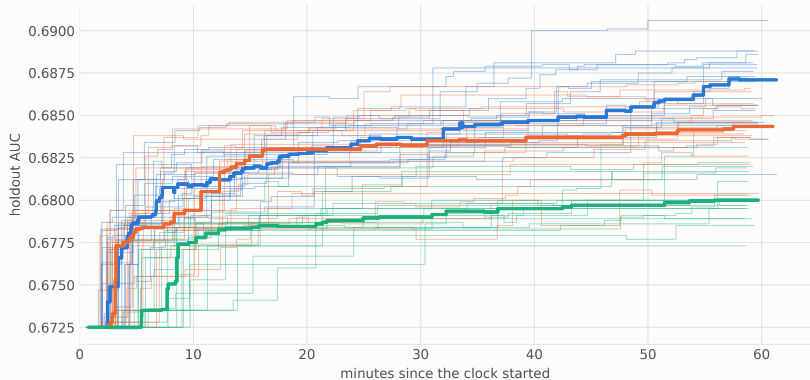
Holdout AUC path per run, median in bold
