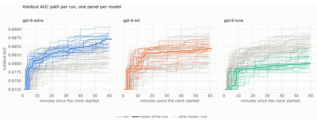
Figure 4: The same paths, one panel per LLM, with the other two LLMs’ runs in grey behind.
