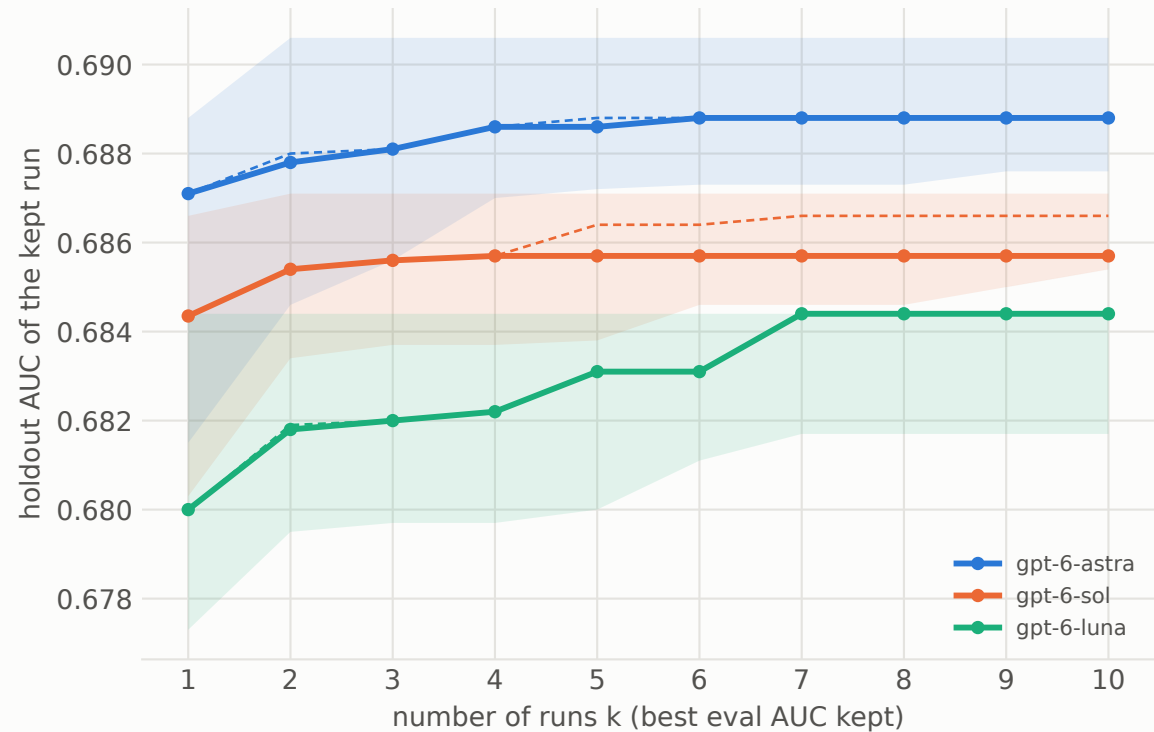
Best of k runs: median (line), 5th to 95th percentile (band), oracle on holdout (dashed)
