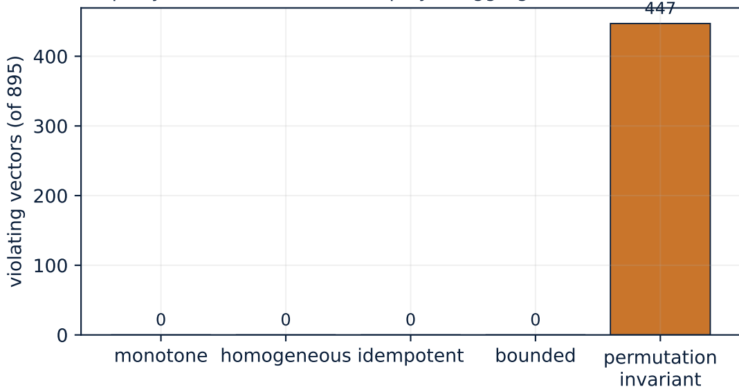
Property conformance of the deployed aggregator
