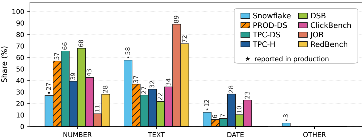
Filter Column Logical Types
