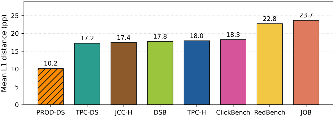
Closeness to Production: Mean L1 Distance per Benchmark
