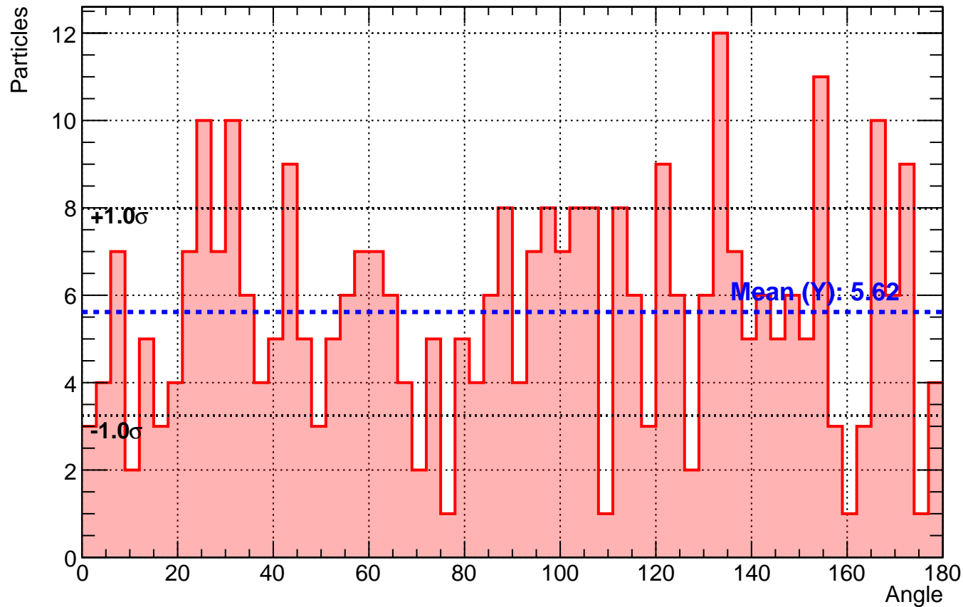
Histogram 4 Coincidances 3 degree
