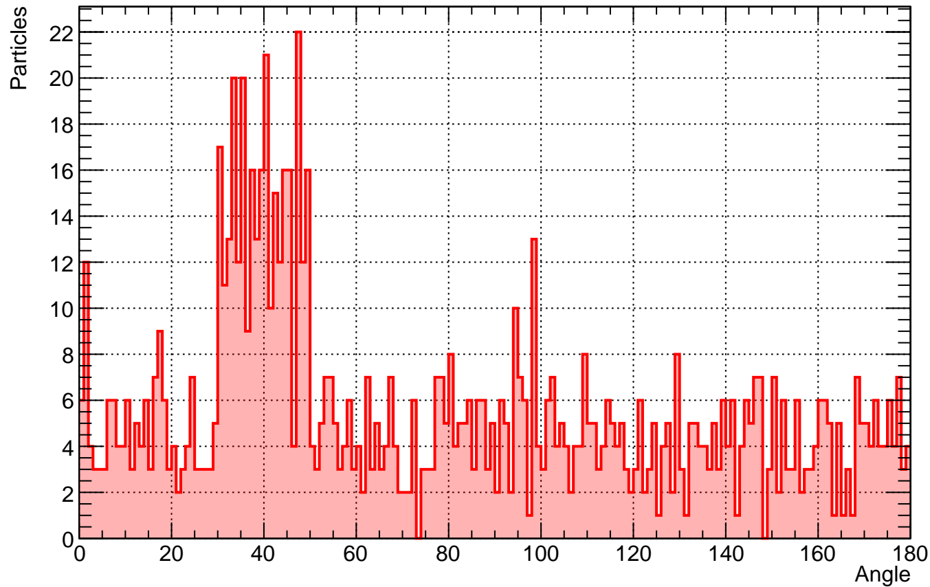
Histogram
