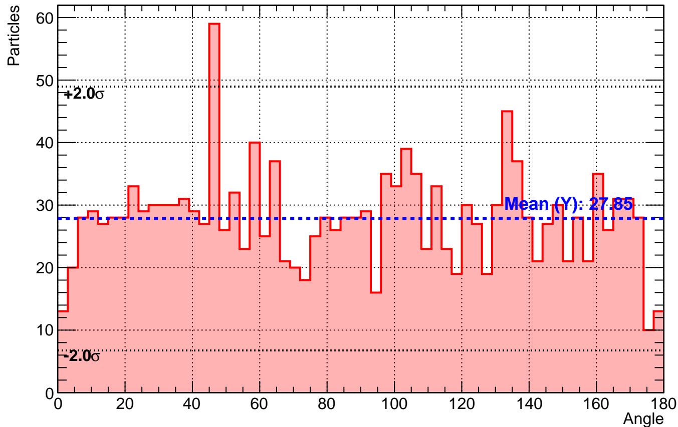
Histogram 34f Coincidences 3 degree
