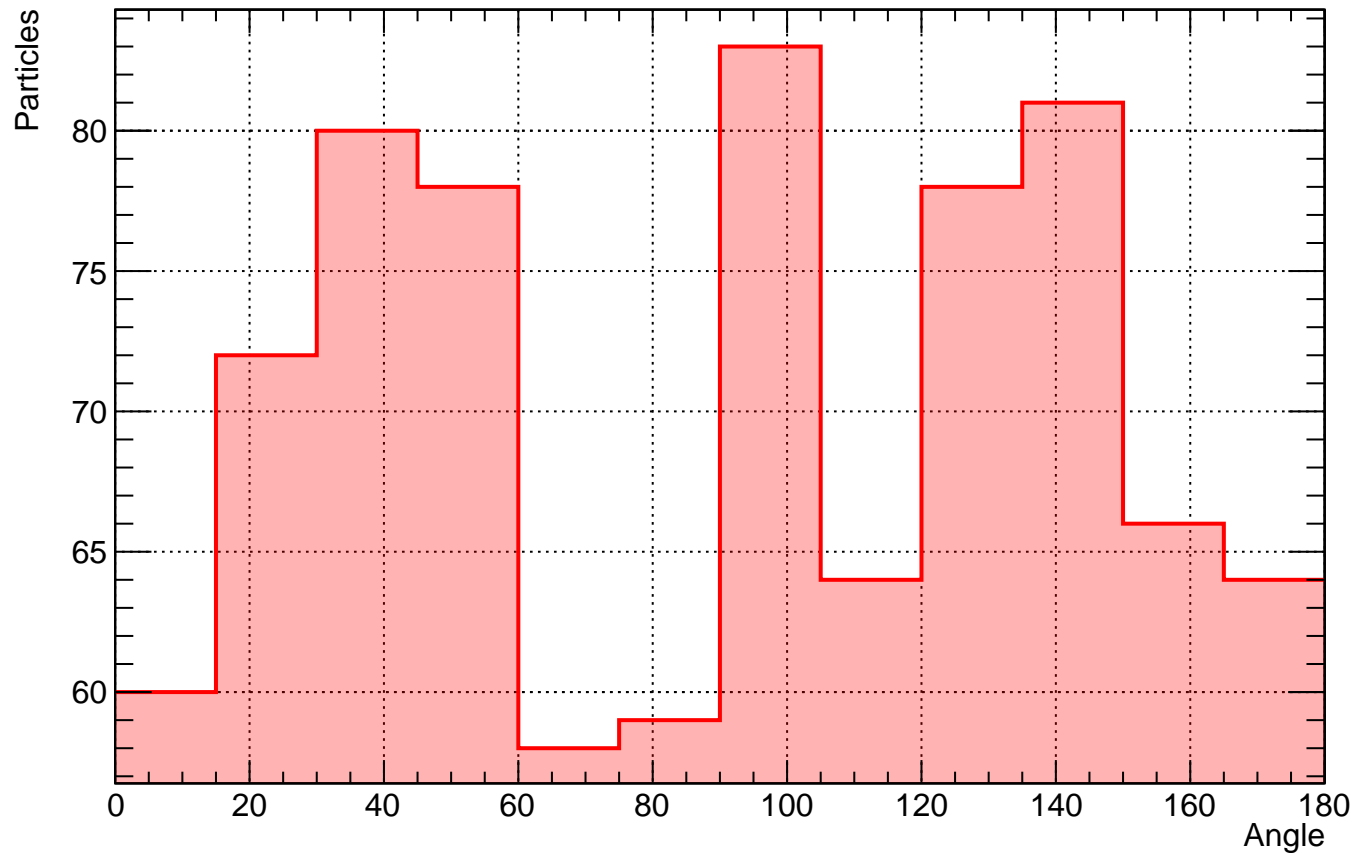
Histogram 3-4 Coincidence 15 degree
