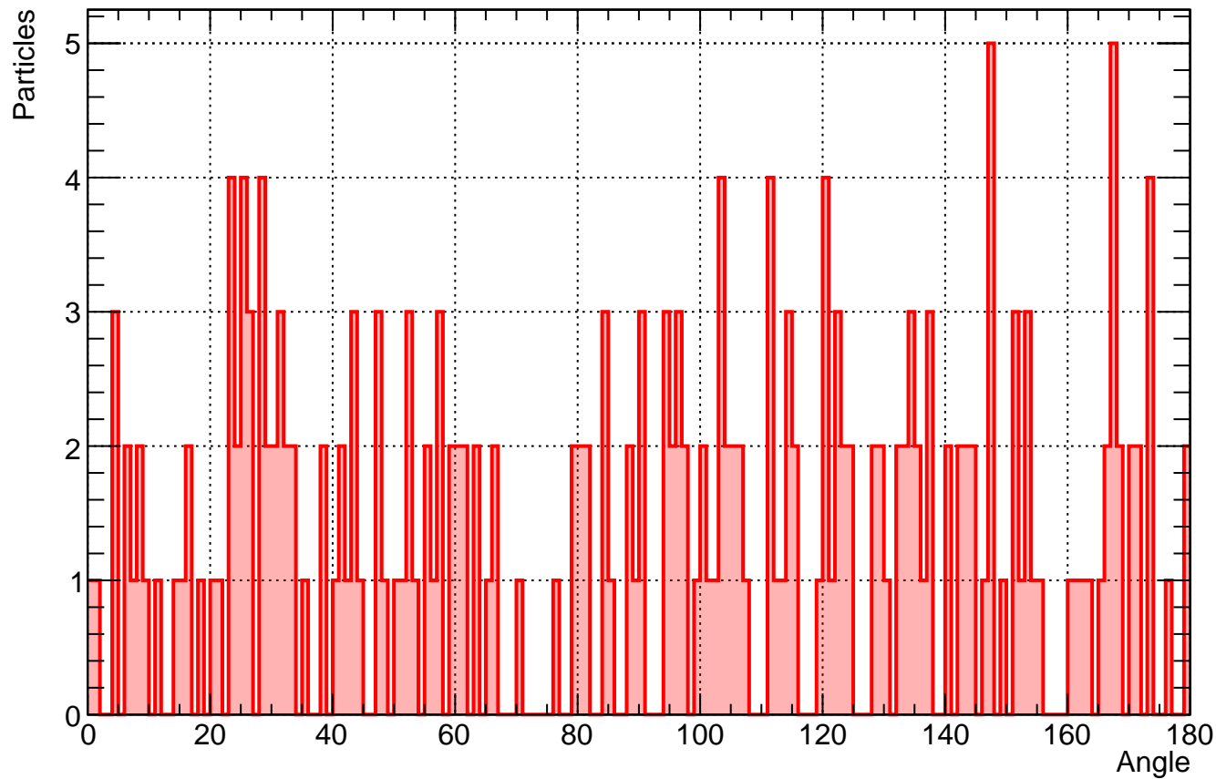
Histogram for 4-coincidences
