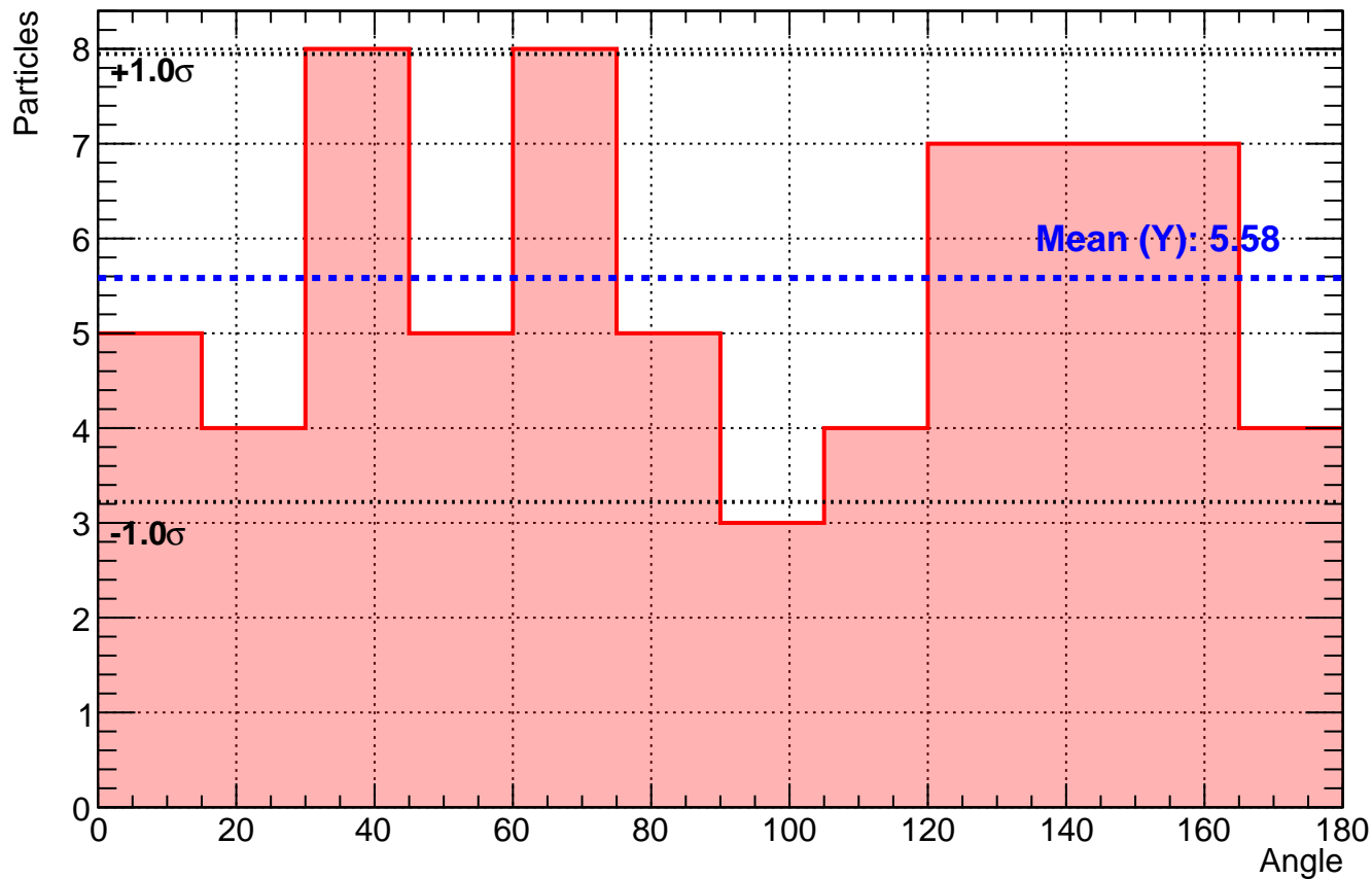
Histogram 4 Coincidences 15 degree
