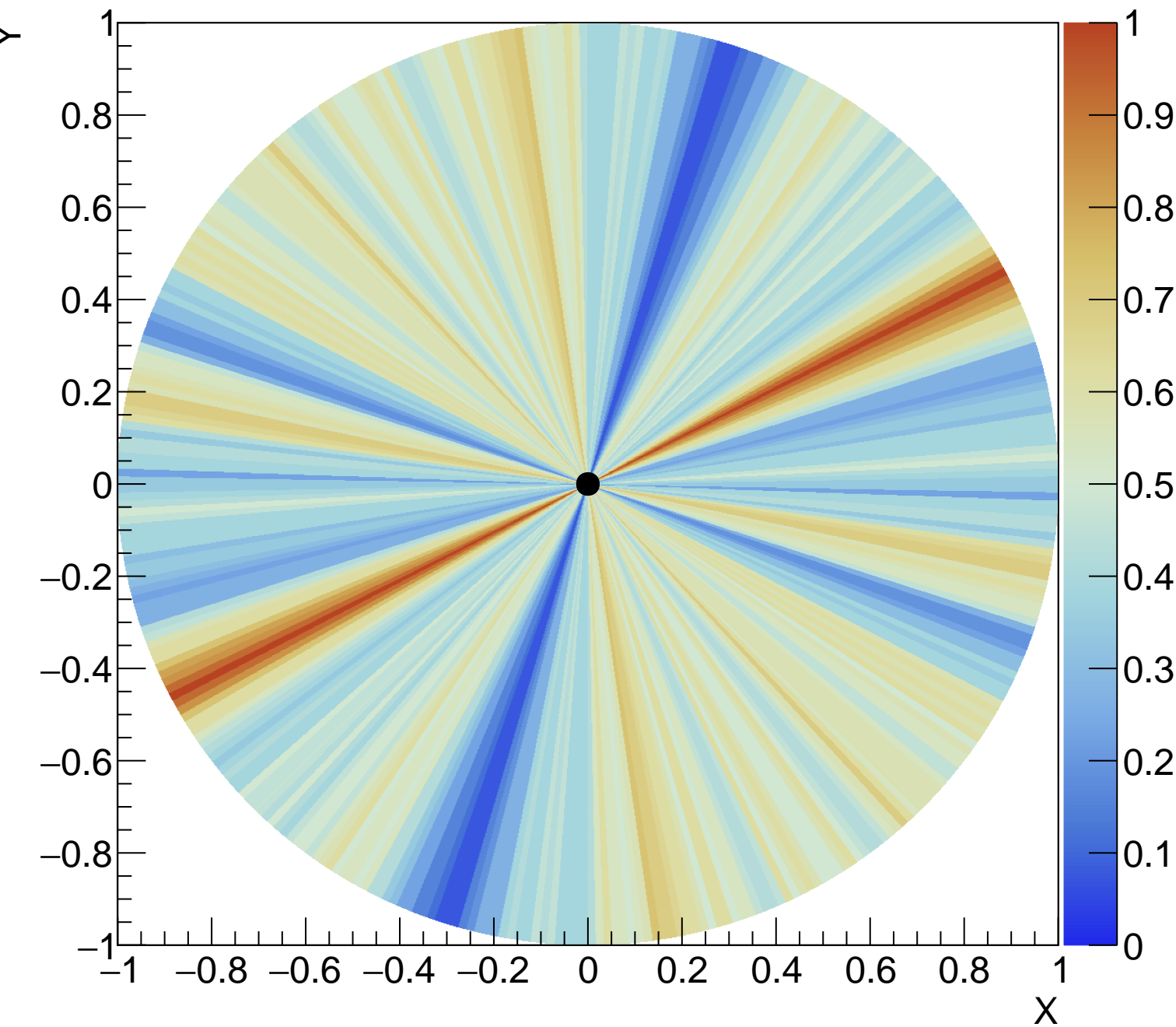
PSF 4 Coincidence 5 degree
