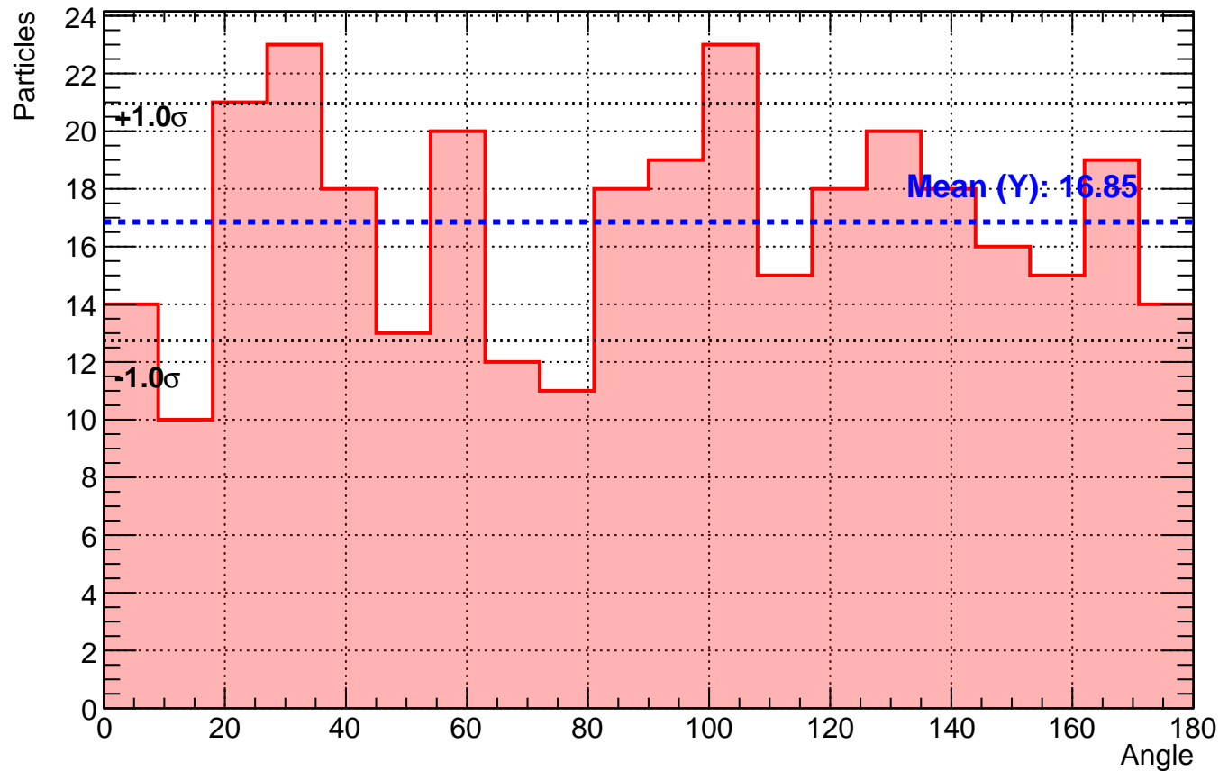
Histogram 4 Coincidances 9 degree
