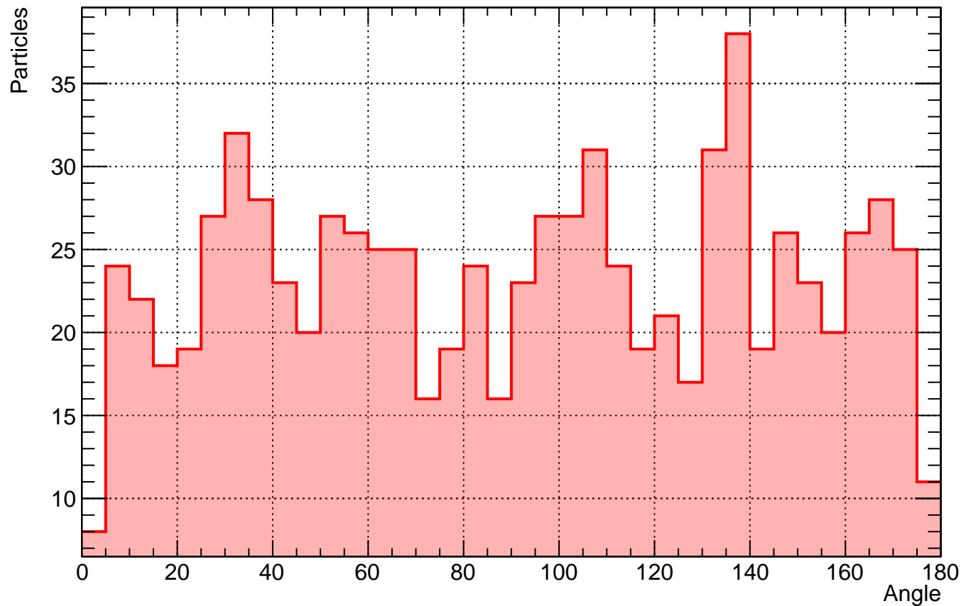
Histogram 3-4 Coincidence
