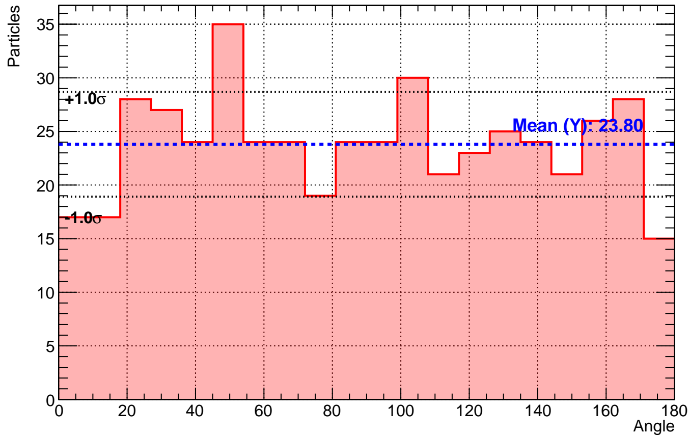
Histogram 4 Coincidences 9 degree
