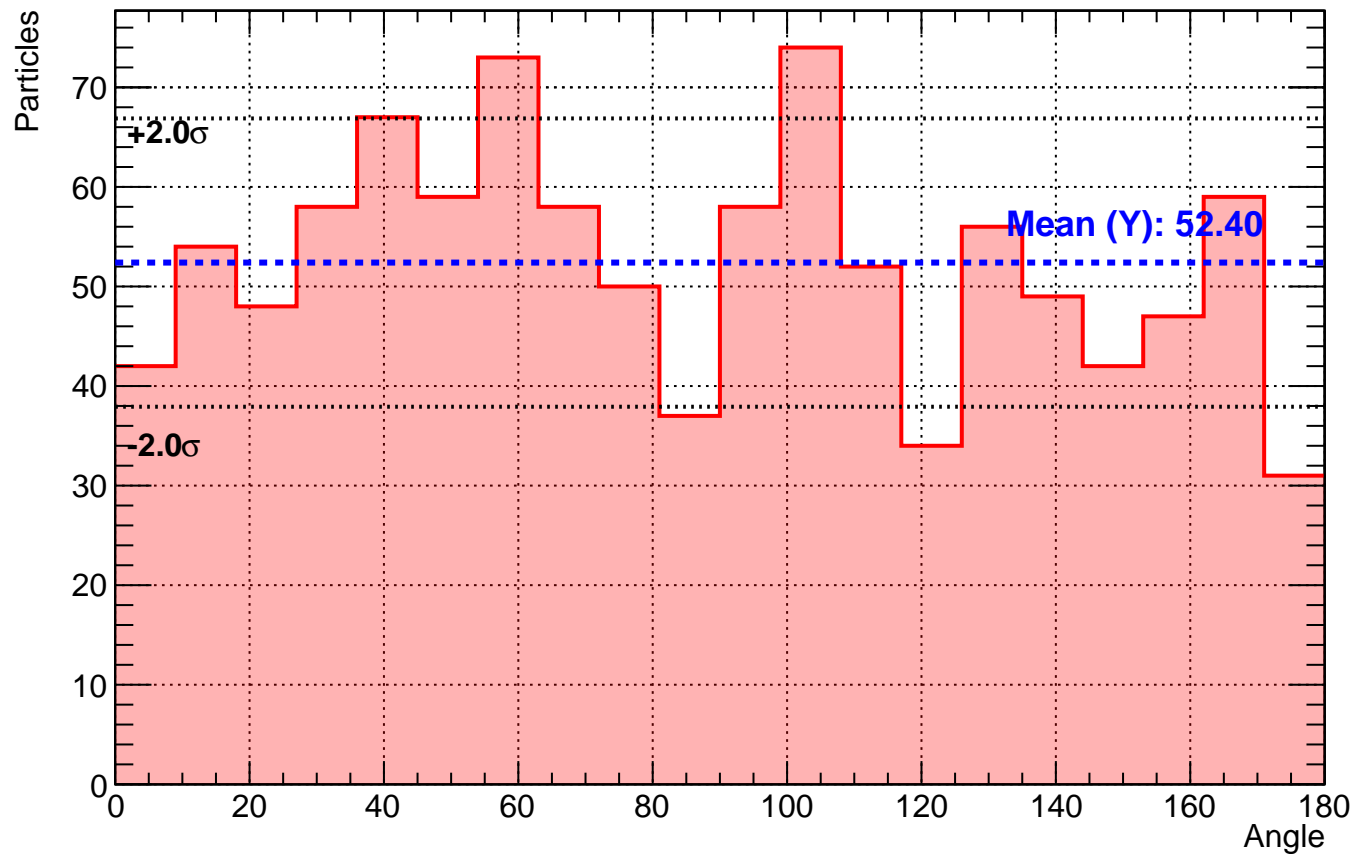
Histogram 1-34 + -234 Coincidances 9 degree
