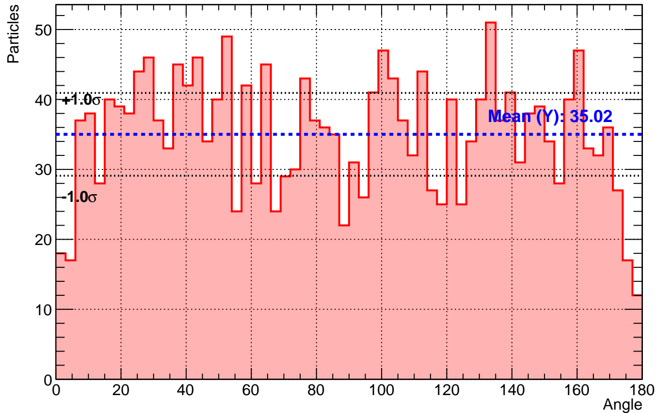
Histogram 3 Coincidences 3 degree
