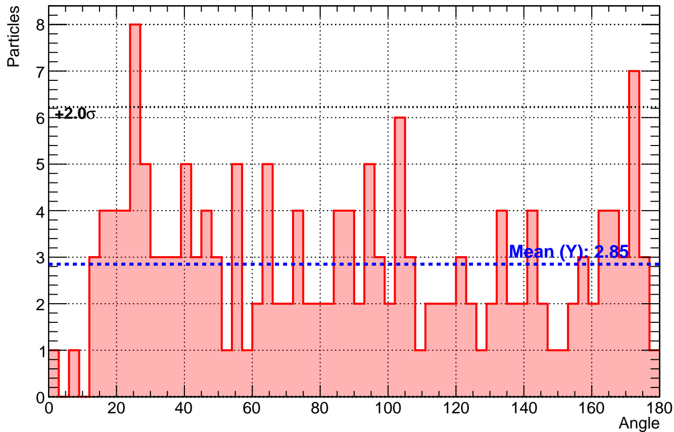
Histogram 34 Coincidences 3 degree
