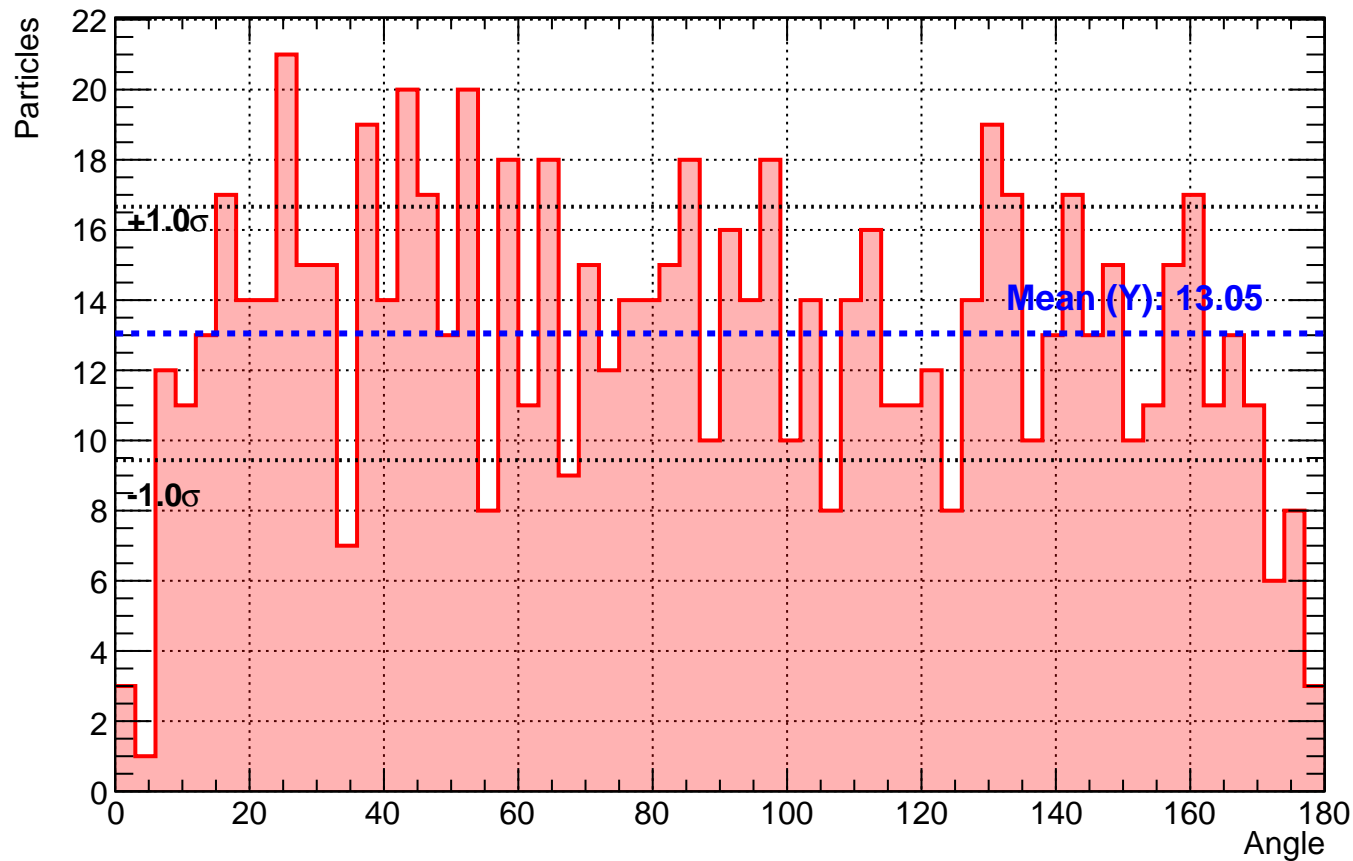
Histogram 3 Coincidences 3 degree
