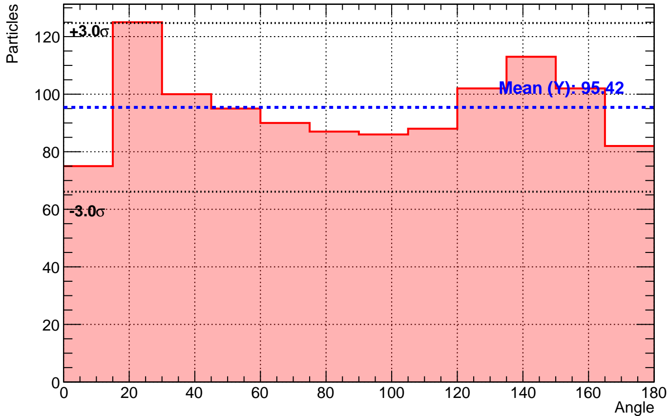
Histogram 123- + 12-4 Coincidances 15 degree
