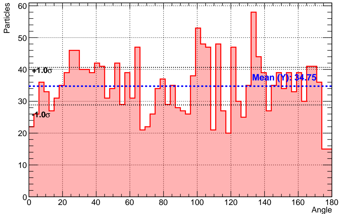
Histogram 3-4 Coincidances 3 degree
