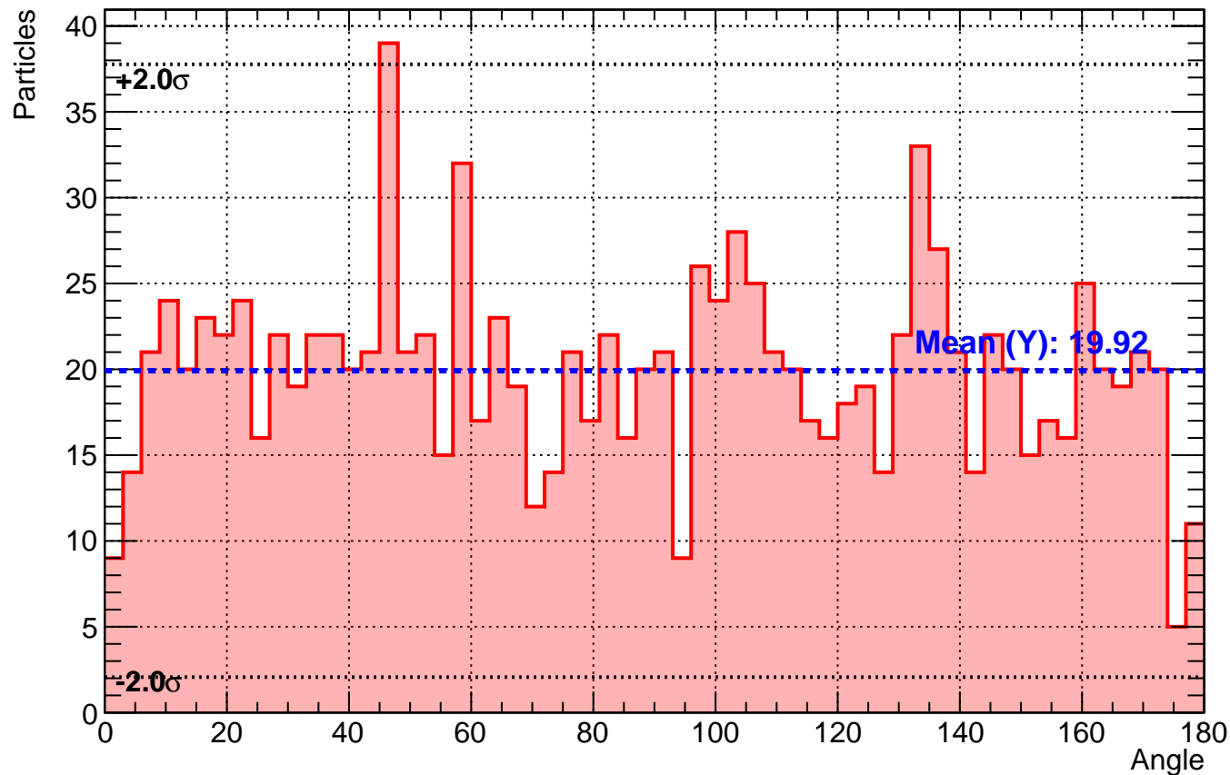
Histogram 3f Coincidences 3 degree
