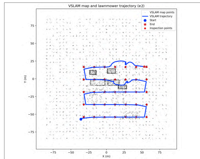
(b) Target VSLAM map and trajectory
