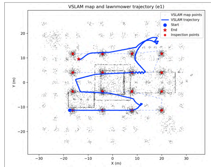
(b) Source VSLAM map and trajectory
