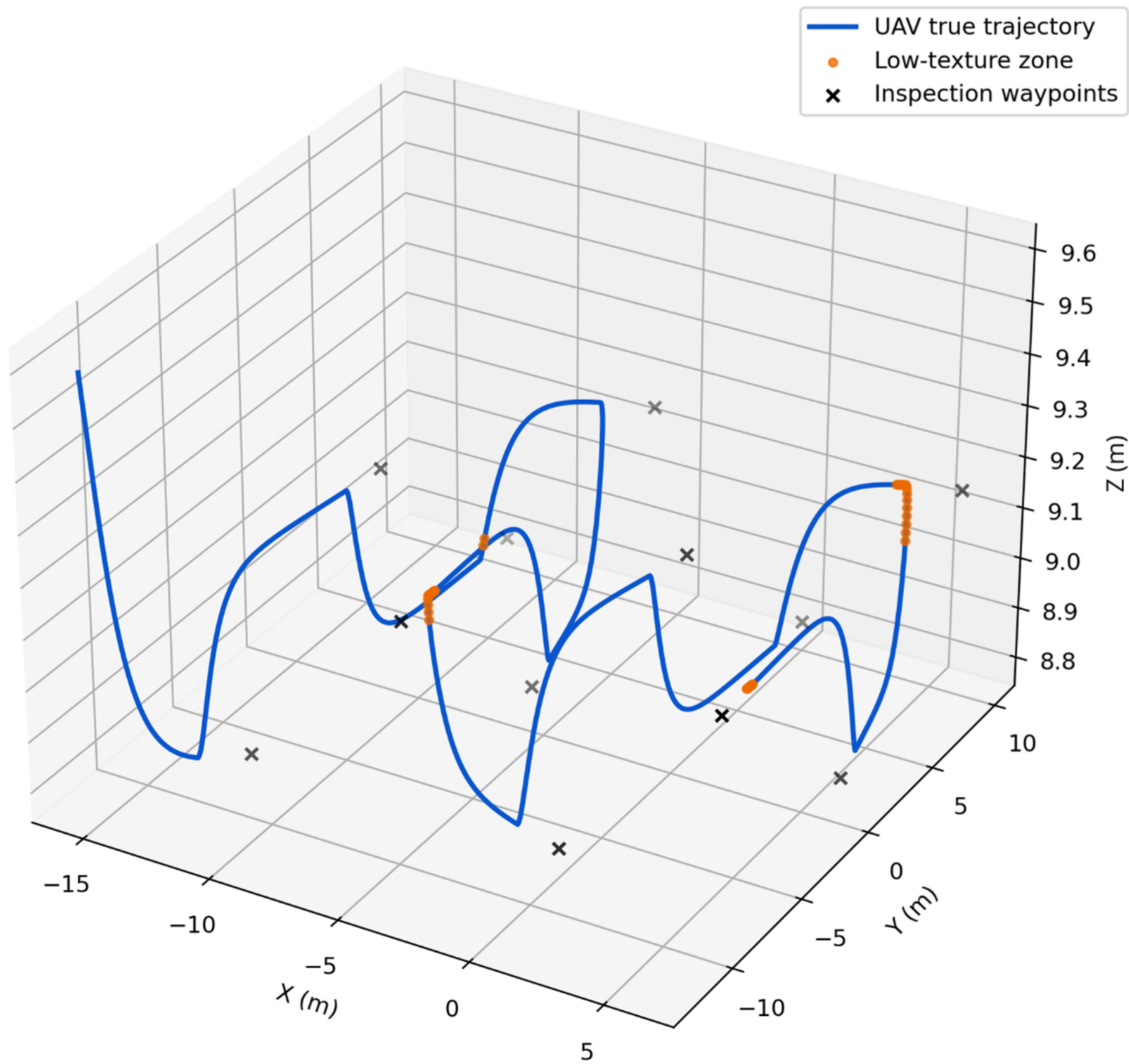
UAV inspection trajectory in 3D (e2)
