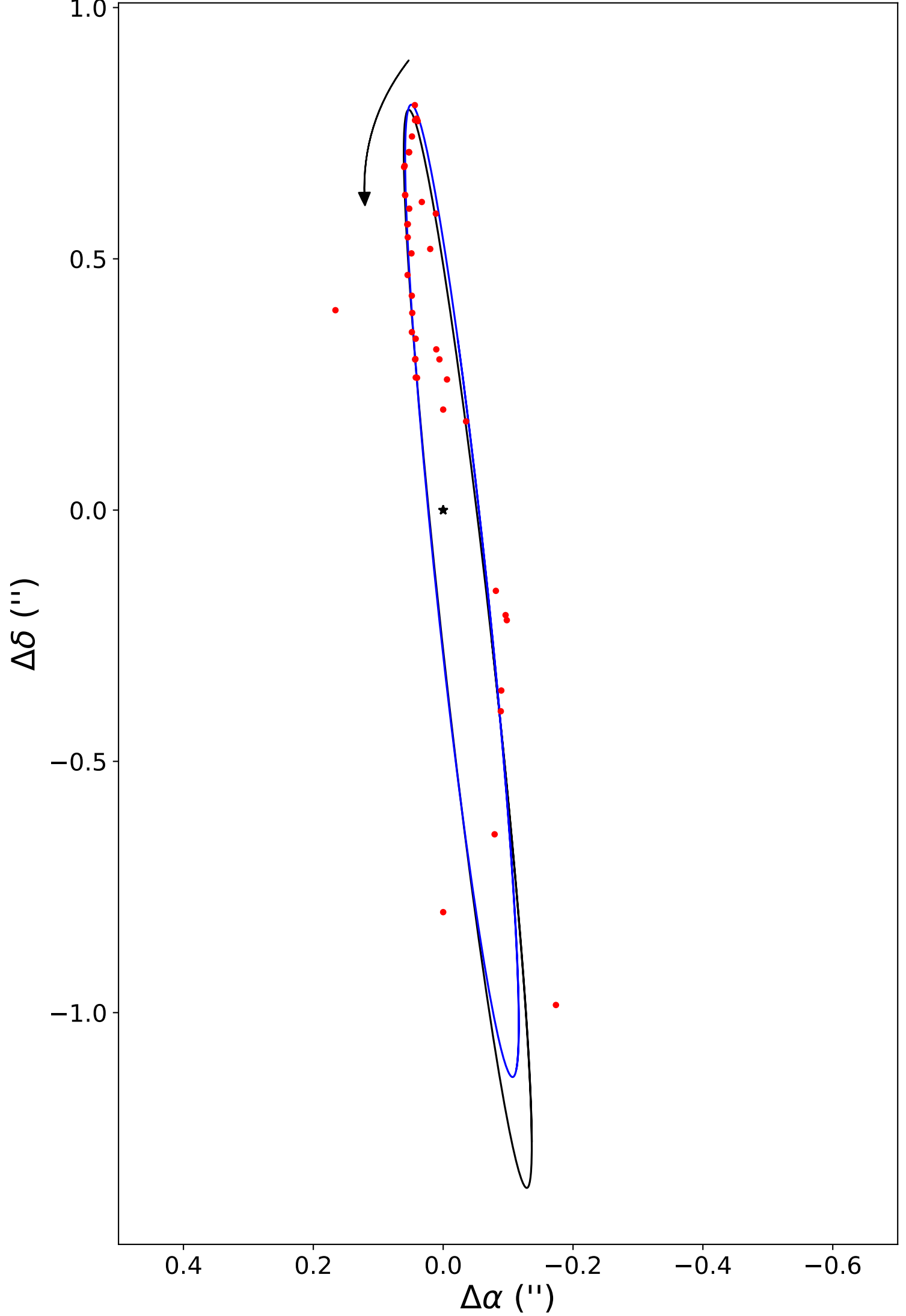
Outer orbit
