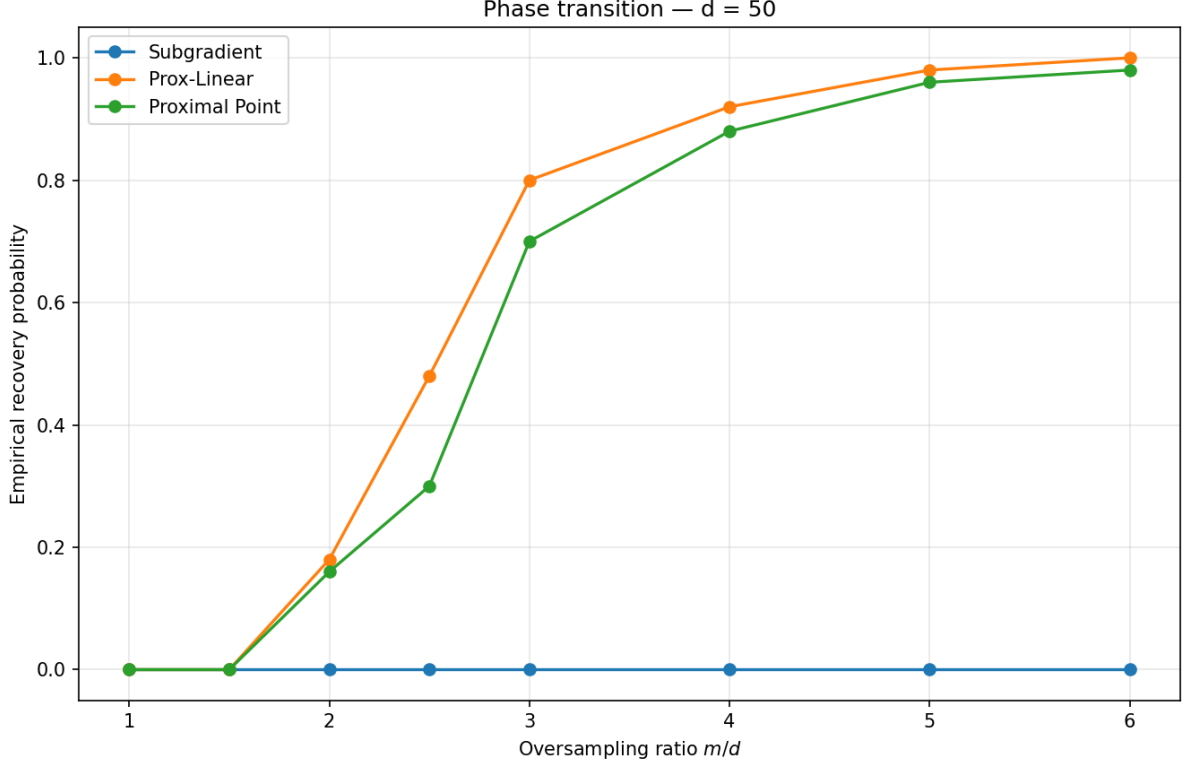
Figure 15: Recovery probability vs. oversampling ratio m/d for the three model-based methods, d = 50 , 50 trials per ratio.
