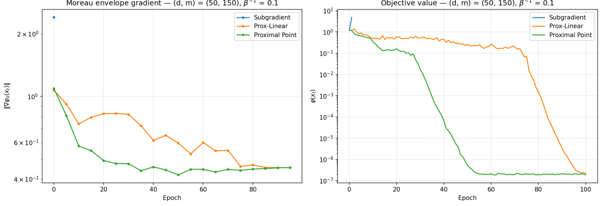
Figure 11: Moreau envelope gradient norm: (d, m) = (50, 150)
