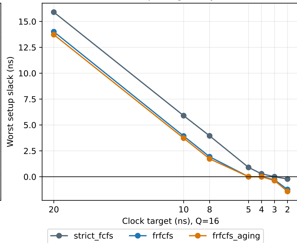
Setup margin only
