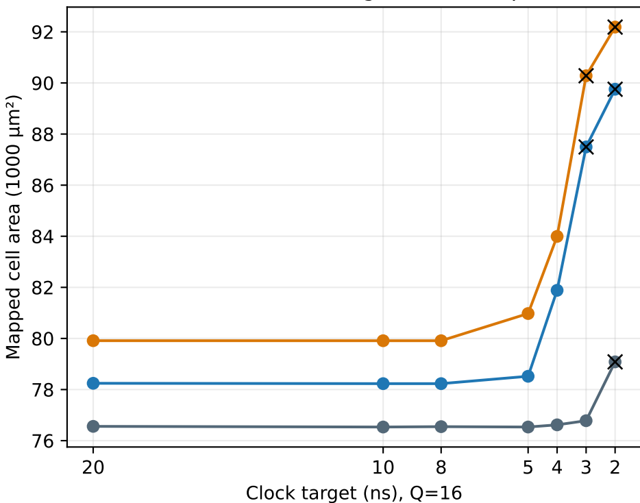
Area versus clock target; × = setup fails
