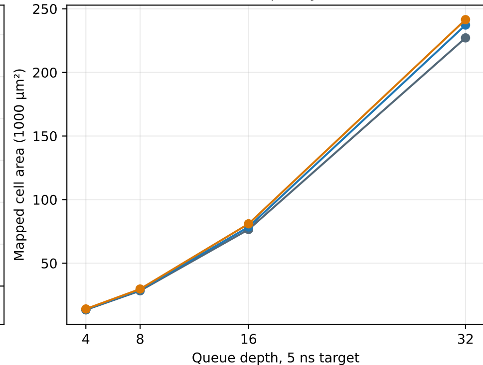
Queue capacity cost
