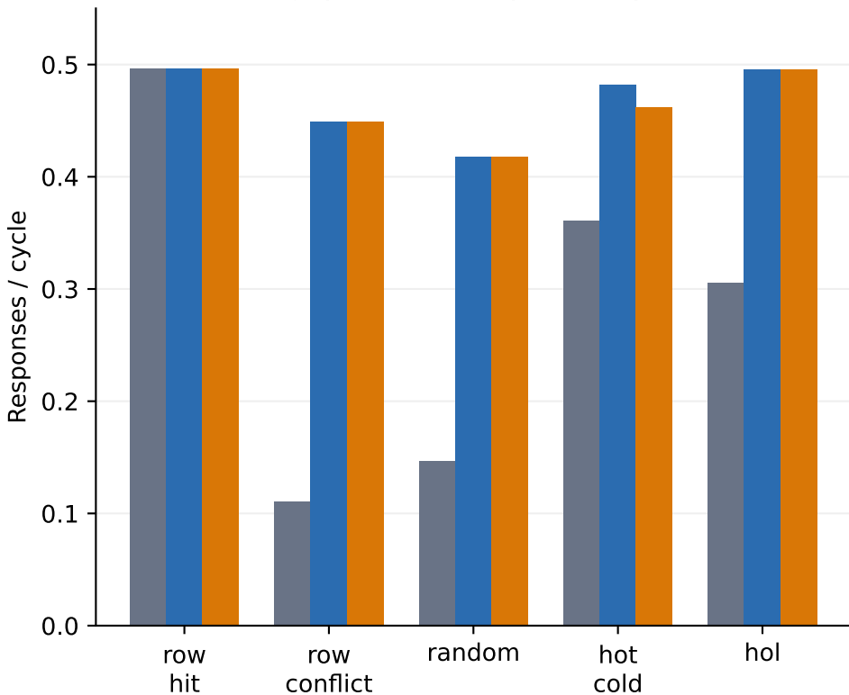
Throughput: fixed request sequences
