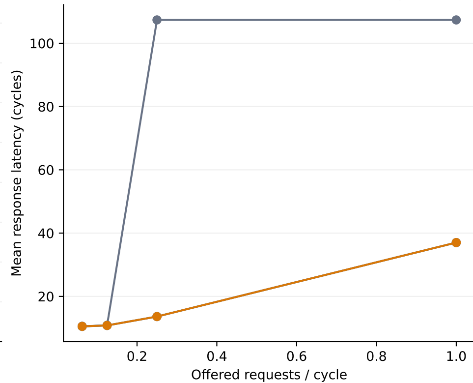
Random traffic: offered-load sweep
