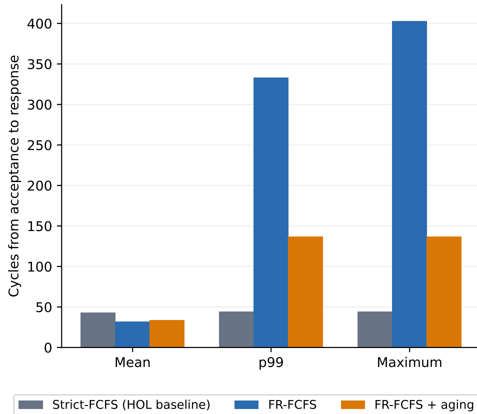
Hot/cold latency: locality versus aging
