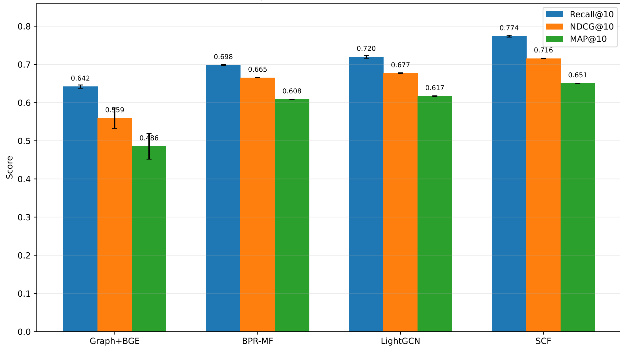
Overall Top-10 Performance on the Full Test Set
