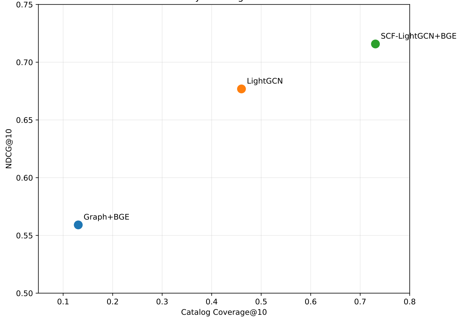
Accuracy-Coverage Tradeoff
