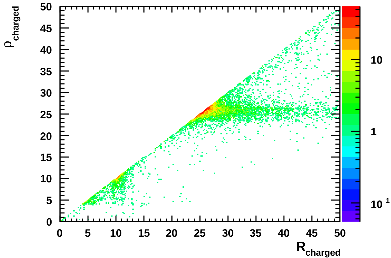
Rho Charged vs R Regeneration
