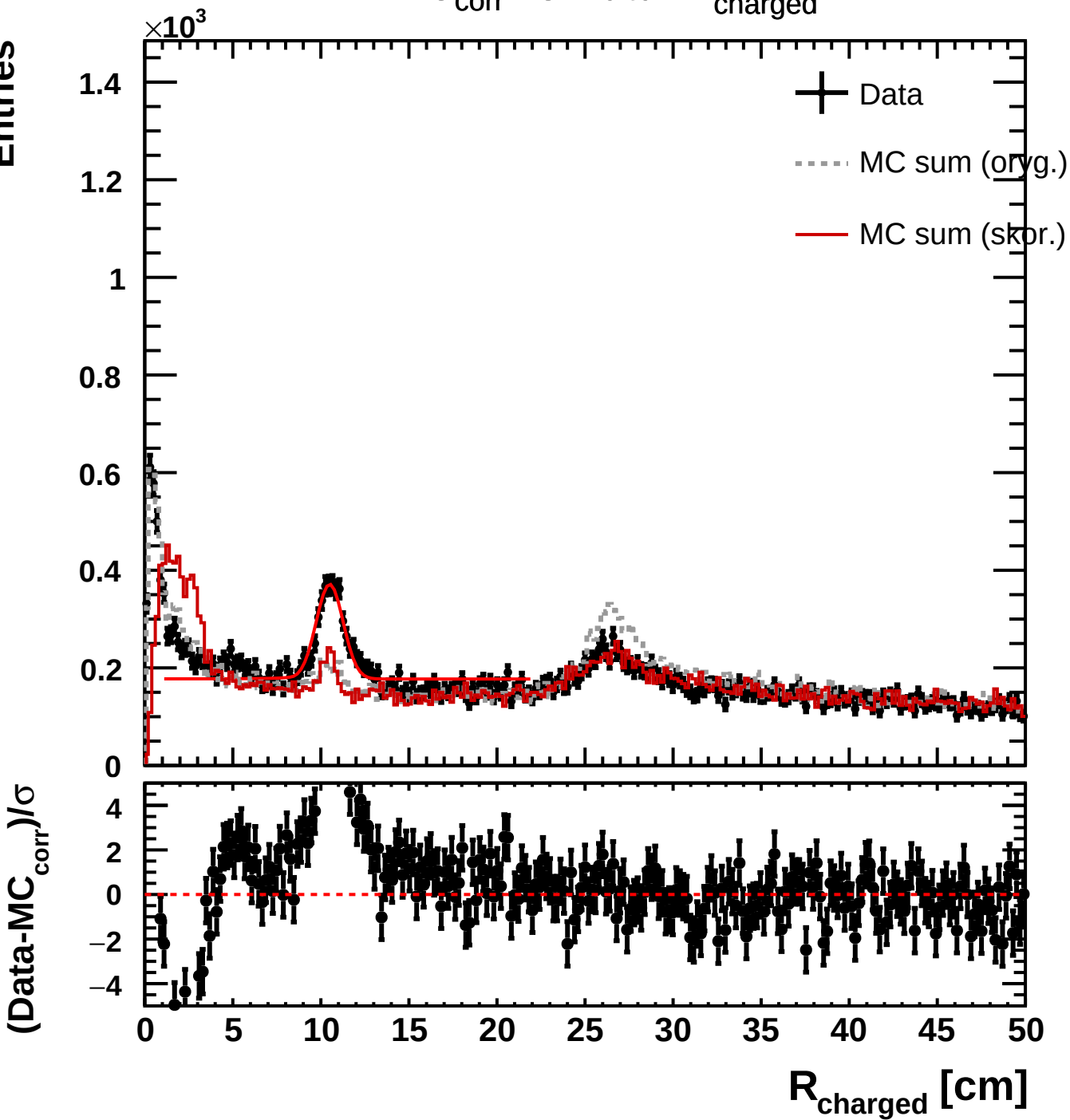
MC corr vs Data: R charged
