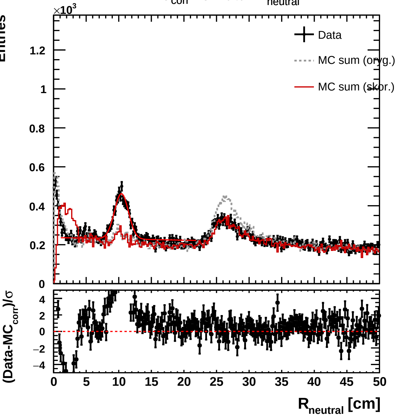
MC corr vs Data: R neutral
