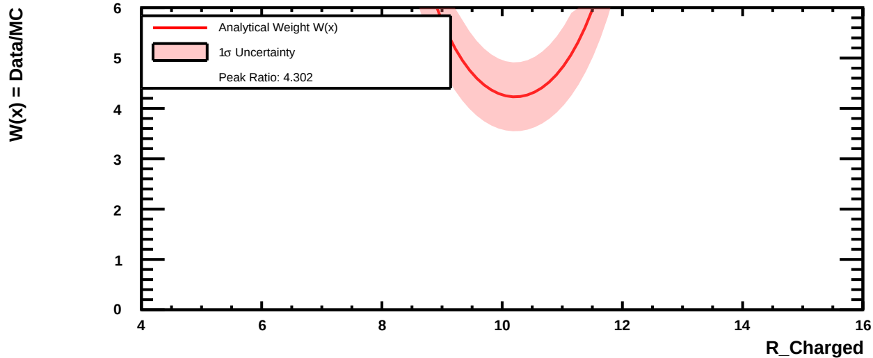
Correction Factor W(R_{\text{Charged}}) with 1\sigma Band
