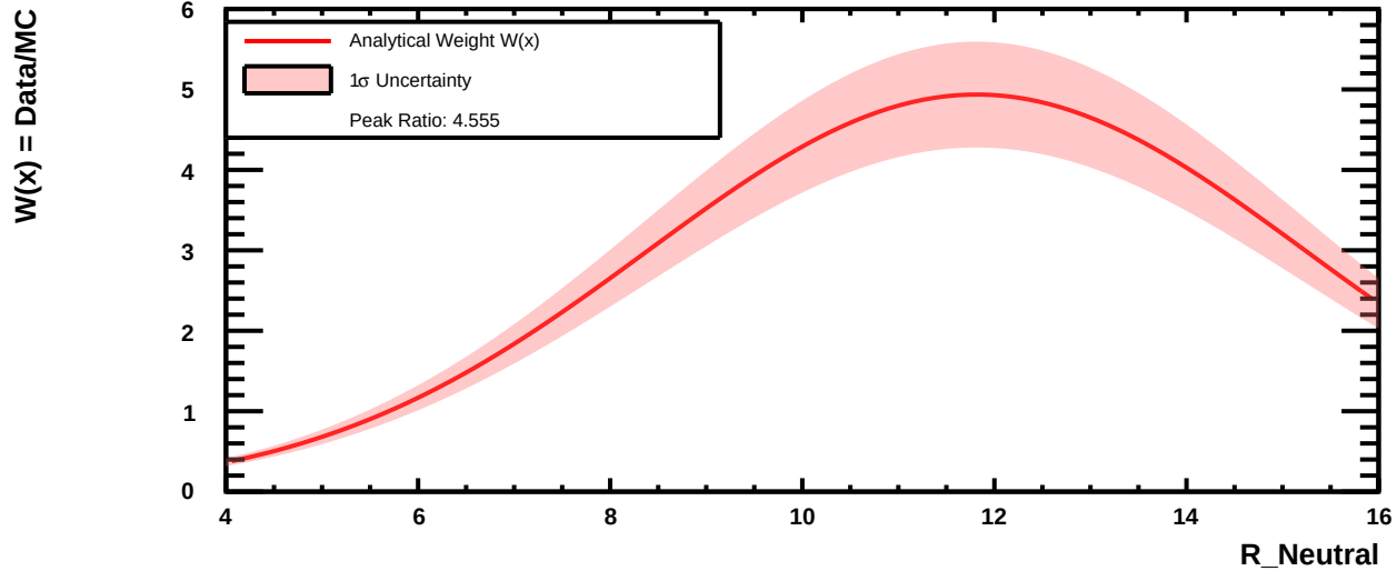
Correction Factor W(R_Neutral) with 1 \sigma Band
