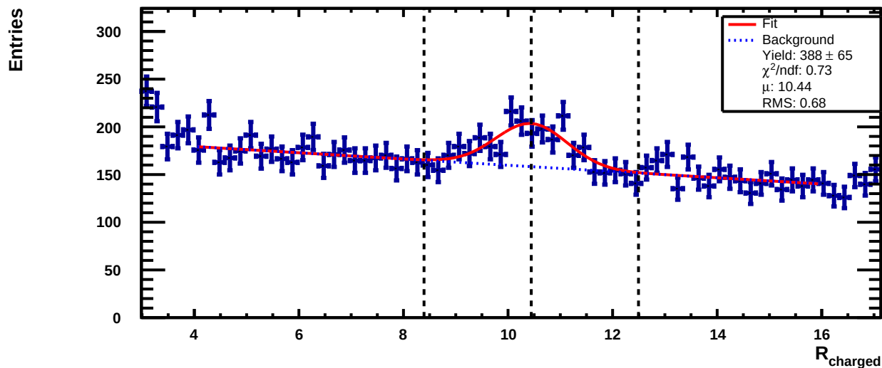
R_Charged (MC SUM)
