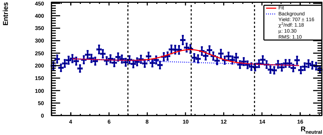
R_Neutral (MC SUM)
