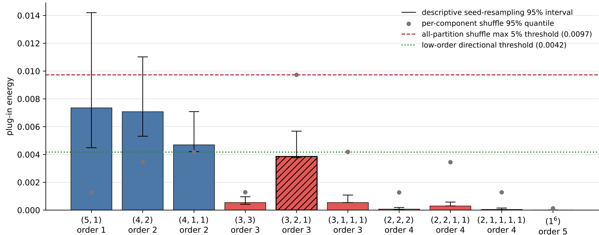
S_6 nontrivial isotypic spectrum of the ten-seed mean landscape
