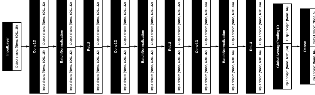
Figure 1: FCN architecture
