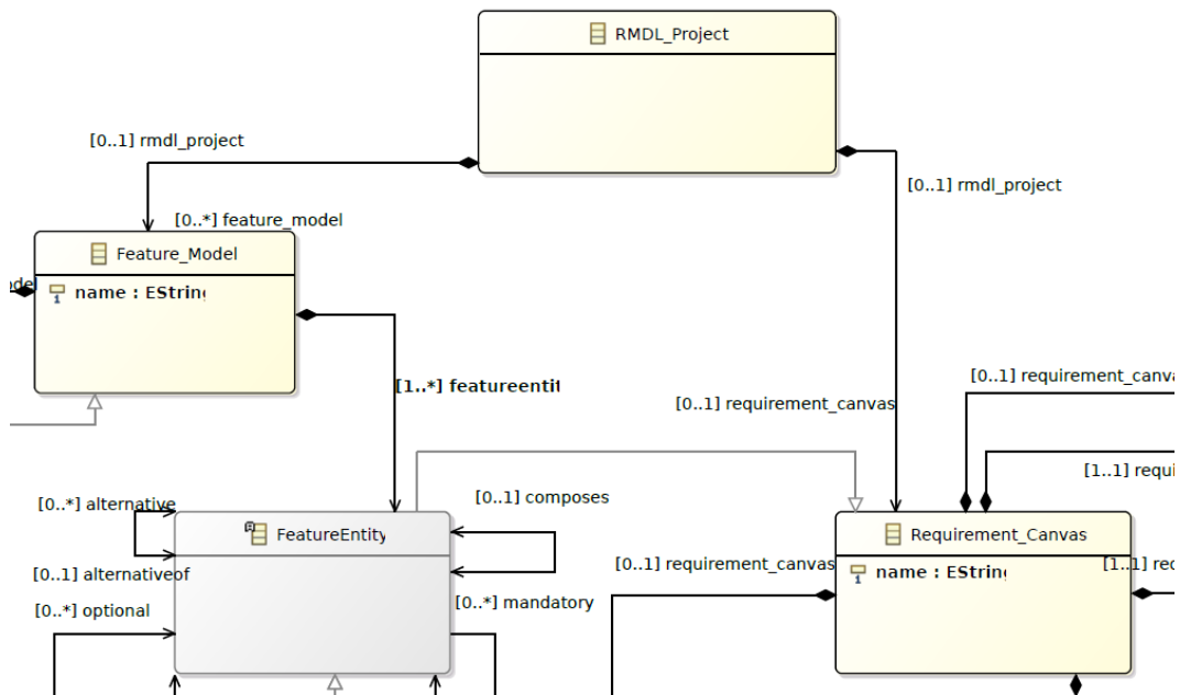
Figure 3.12: CyclicL metamodel. Shows the specification relationship between the requirement canvas and feature modelling portions of the metamodel. Also shows their relation to the model root.
