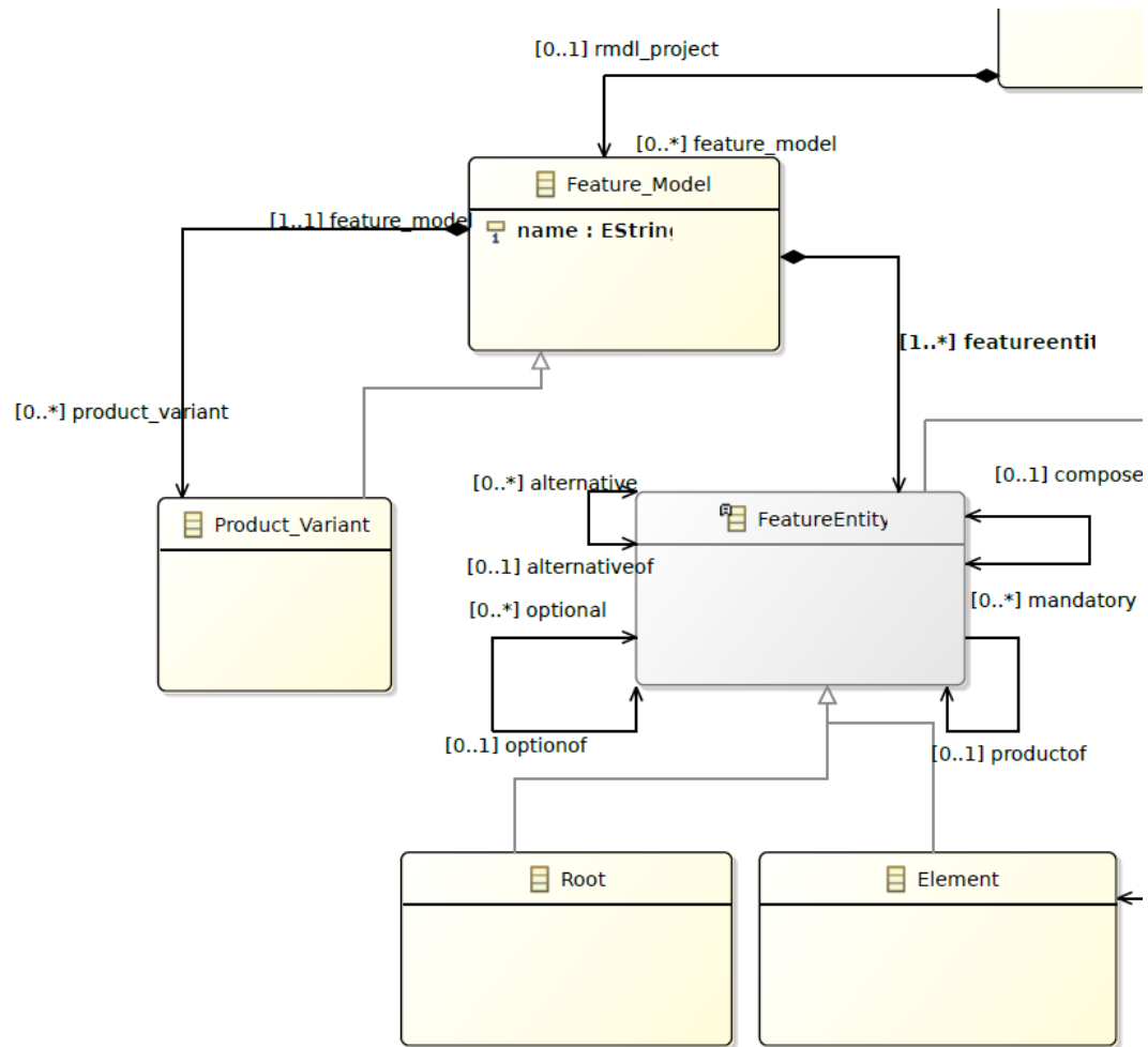
Figure 3.9: CyclicL metamodel. Shows the specification for the feature modelling portion of CyclicL.
