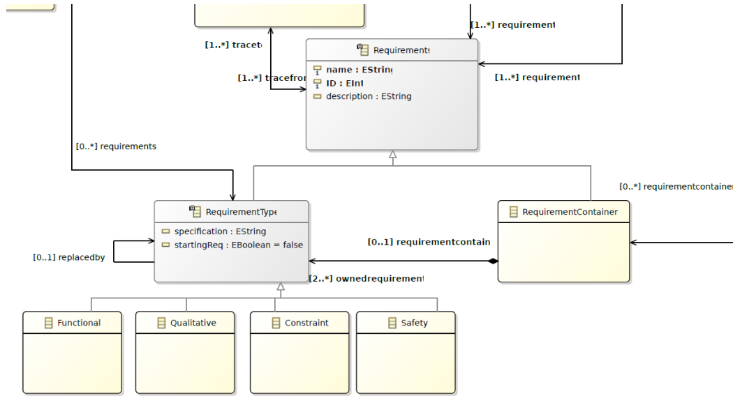
Figure 3.11: CyclicL metamodel. Shows the specification for the second half of the requirement canvas portion of CyclicL.
