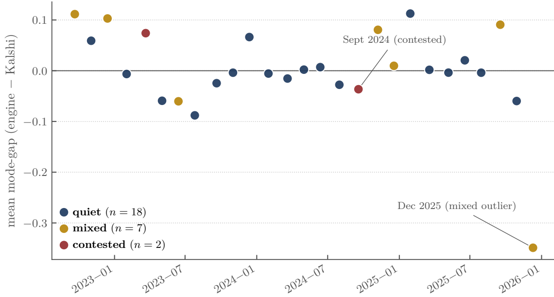
Figure 3: Per-meeting mean window mode-gap, by regime, on the primary n = 27 sample. Each point is one FOMC. Quiet meetings cluster tightly around zero; the seven mixed meetings span -0.349 (fed_2025-12-10, the largest distributional gap in the sample) to +0.11 . The two contested meetings (March 2023, September 2024) sit close to zero with the engine slightly more concentrated on the realized bucket in March 2023 and slightly less in September 2024.
