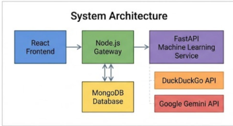
Fig. 1. High-Level System Architecture and Multi-Tier Orchestration Network of the NewsPulse-AI Platform.
