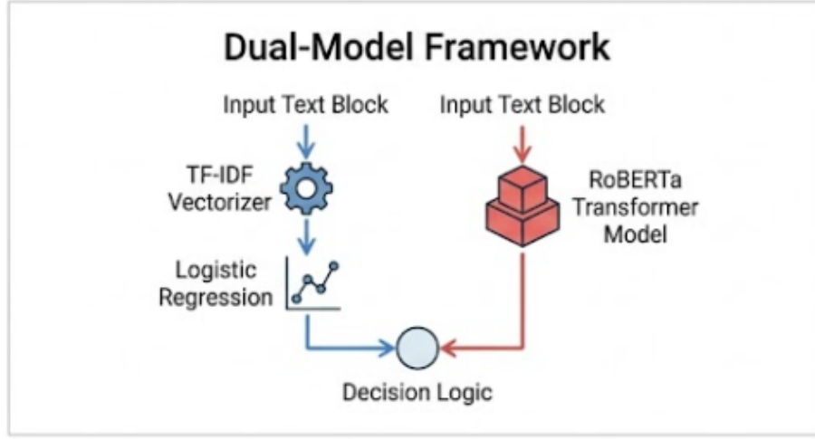
Fig. 4. Dual-Engine Parallel Machine Learning Architecture inside NewsPulse-AI.
