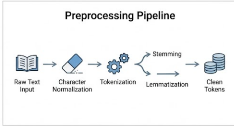
Fig. 3. Sequential Text Tokenization and Linguistic Preprocessing Pipeline for NewsPulse-AI.
