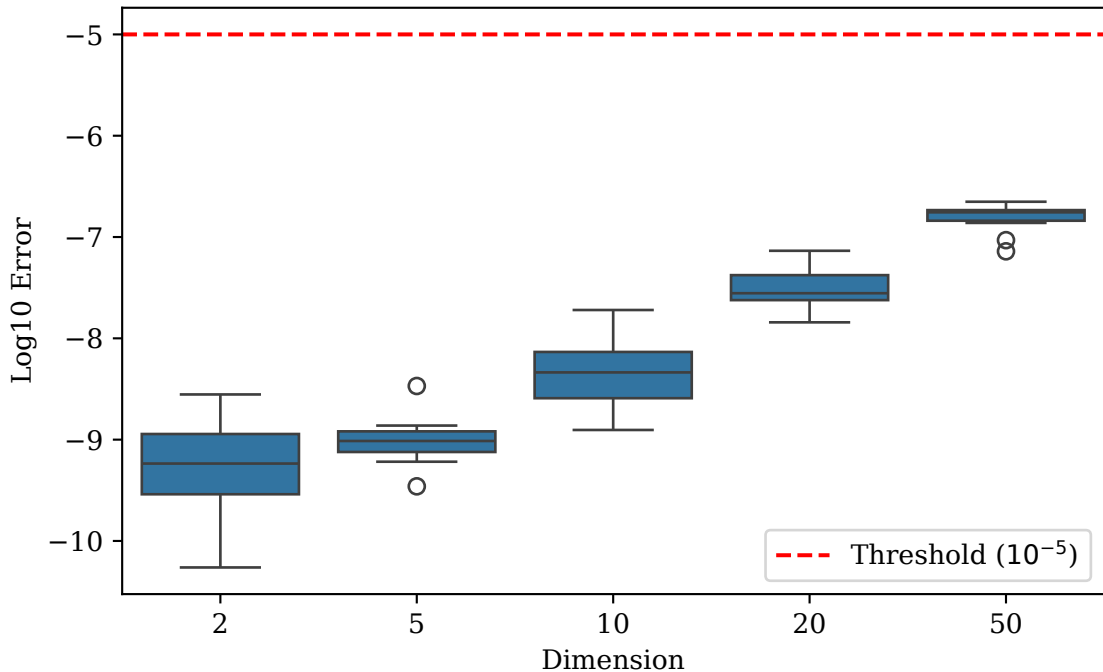
Gradient Verification: Relative Error Distribution
